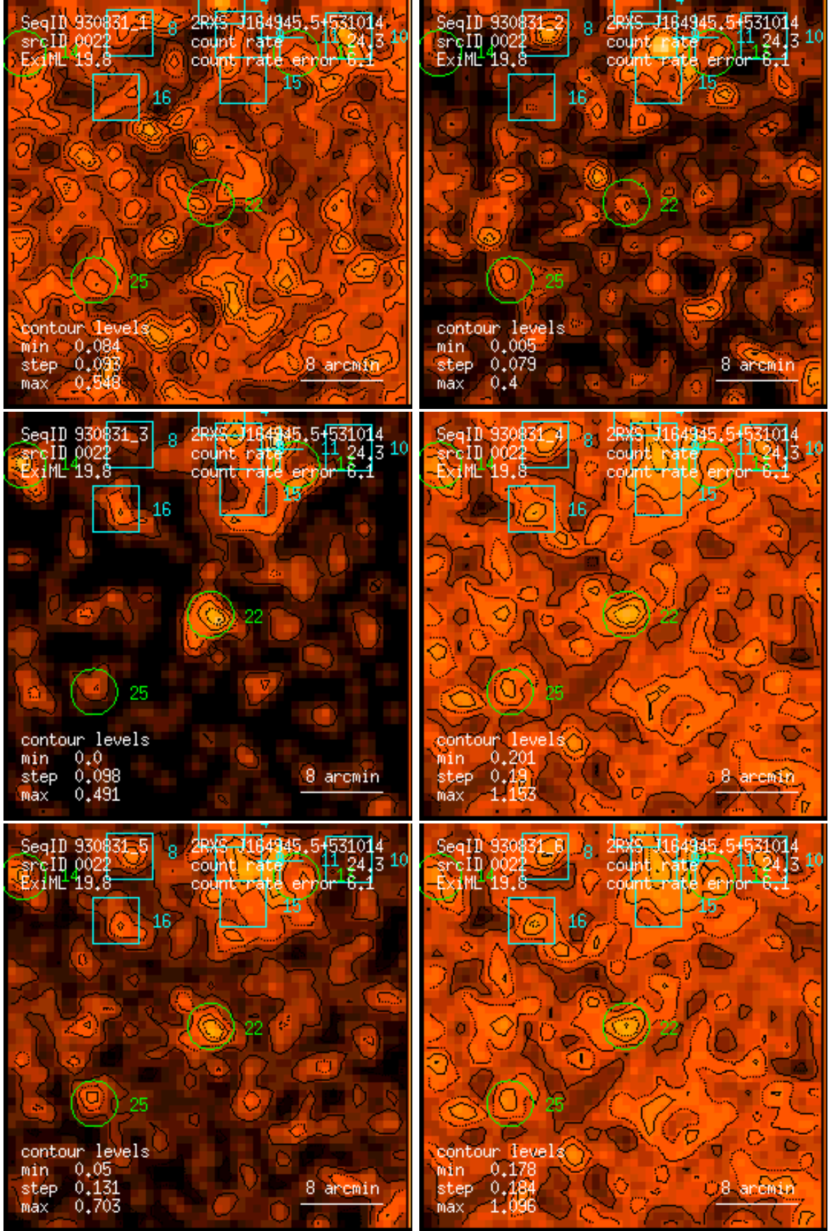
Figure 22: RASS 930831: detection 0022: band rate images, Gaussian filter: (1) PSPC channels 11 – 41, (2) 52 – 90, (3) 91 – 201, (4) 11 – 235, (5) 52 – 201, (6) 11 – 201. Broad band rates in counts/ks. Band rate contour levels in counts/ks/arcmin 2 .
