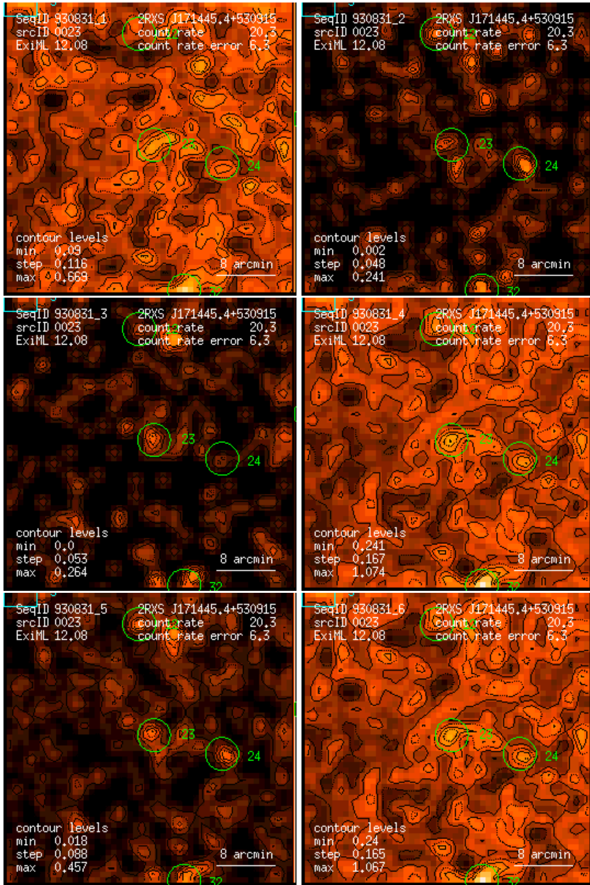
Figure 23: RASS 930831: detection 0023: band rate images, Gaussian filter: (1) PSPC channels 11 – 41, (2) 52 – 90, (3) 91 – 201, (4) 11 – 235, (5) 52 – 201, (6) 11 – 201. Broad band rates in counts/ks. Band rate contour levels in counts/ks/arcmin 2 .
