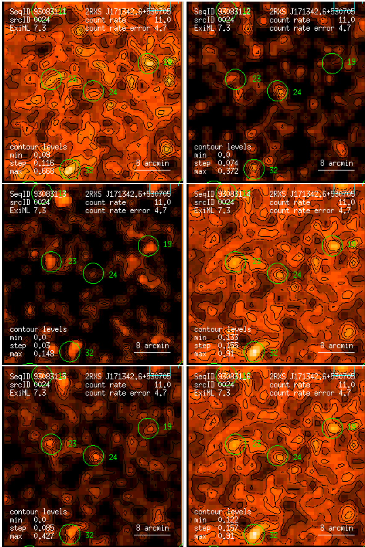
Figure 24: RASS 930831: detection 0024: band rate images, Gaussian filter: (1) PSPC channels 11 – 41, (2) 52 – 90, (3) 91 – 201, (4) 11 – 235, (5) 52 – 201, (6) 11 – 201. Broad band rates in counts/ks. Band rate contour levels in counts/ks/arcmin 2 .
