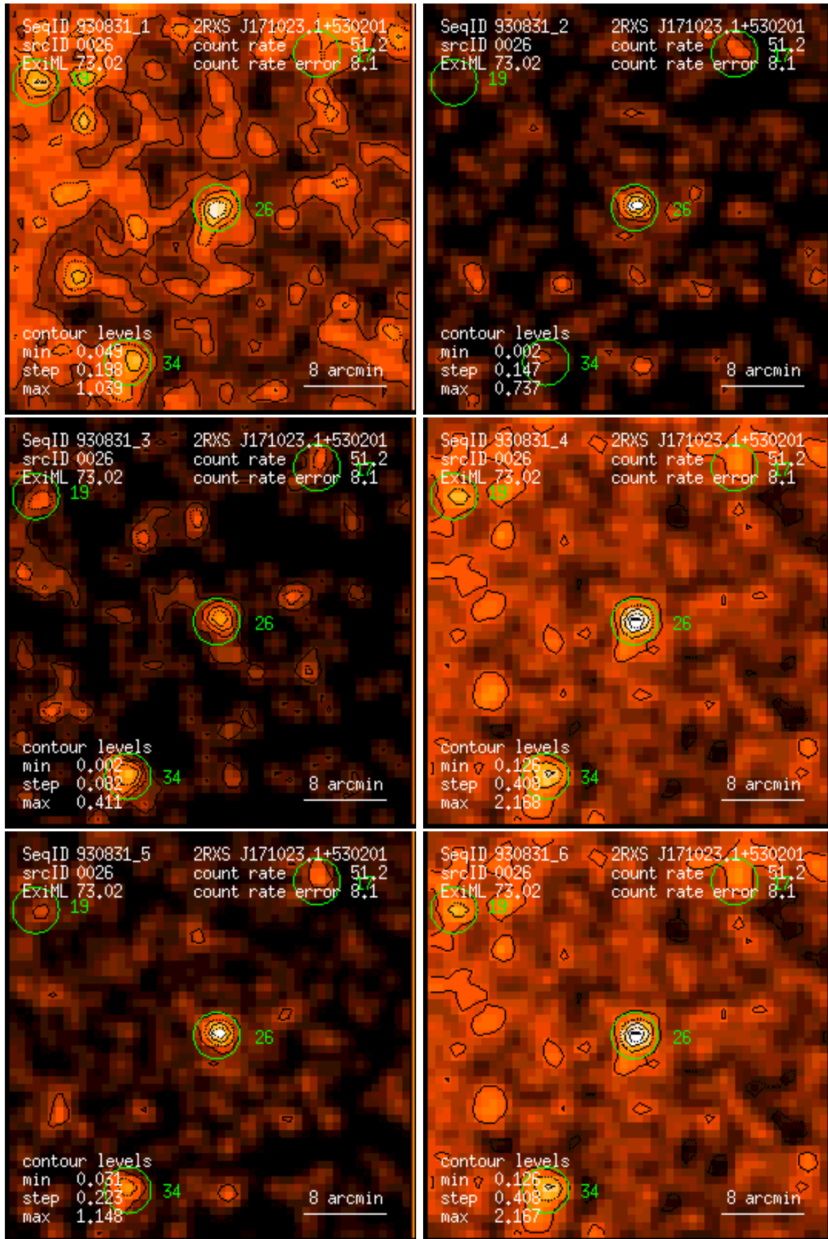
Figure 26: RASS 930831: detection 0026: band rate images, Gaussian filter: (1) PSPC channels 11 – 41, (2) 52 – 90, (3) 91 – 201, (4) 11 – 235, (5) 52 – 201, (6) 11 – 201. Broad band rates in counts/ks. Band rate contour levels in counts/ks/arcmin 2 .
