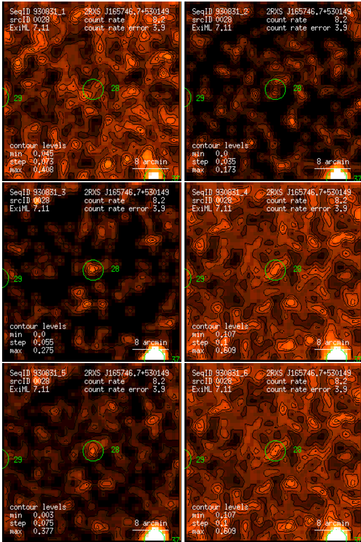
Figure 28: RASS 930831: detection 0028: band rate images, Gaussian filter: (1) PSPC channels 11 – 41, (2) 52 – 90, (3) 91 – 201, (4) 11 – 235, (5) 52 – 201, (6) 11 – 201. Broad band rates in counts/ks. Band rate contour levels in counts/ks/arcmin 2 .
