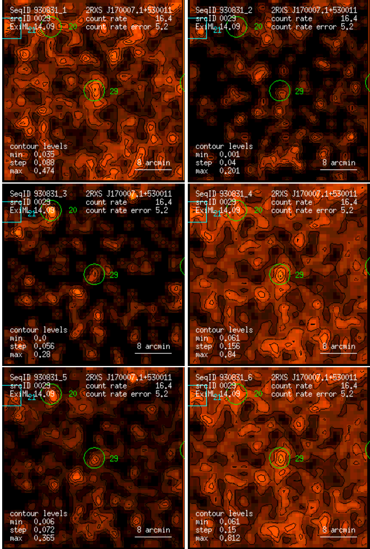
Figure 29: RASS 930831: detection 0029: band rate images, Gaussian filter: (1) PSPC channels 11 – 41, (2) 52 – 90, (3) 91 – 201, (4) 11 – 235, (5) 52 – 201, (6) 11 – 201. Broad band rates in counts/ks. Band rate contour levels in counts/ks/arcmin 2 .
