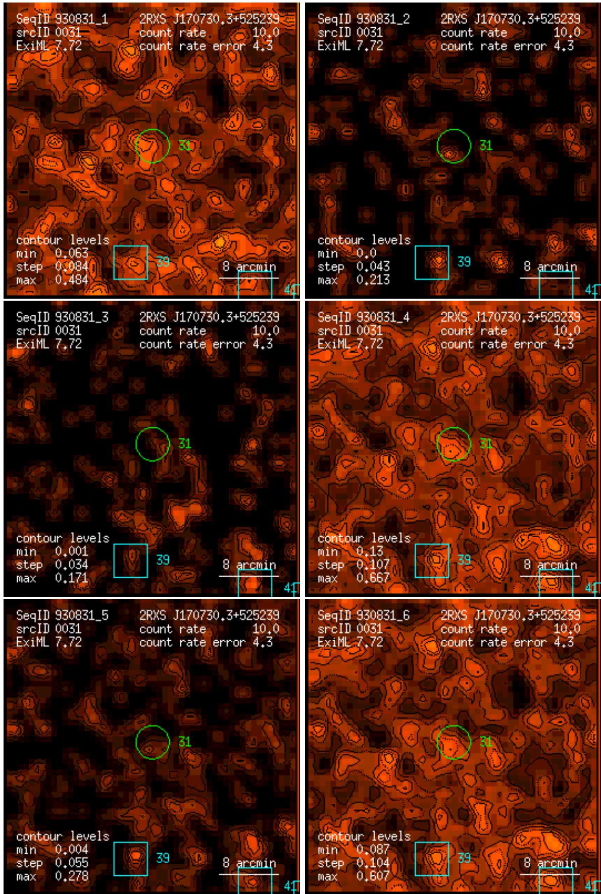
Figure 31: RASS 930831: detection 0031: band rate images, Gaussian filter: (1) PSPC channels 11 – 41, (2) 52 – 90, (3) 91 – 201, (4) 11 – 235, (5) 52 – 201, (6) 11 – 201. Broad band rates in counts/ks. Band rate contour levels in counts/ks/arcmin 2 .
