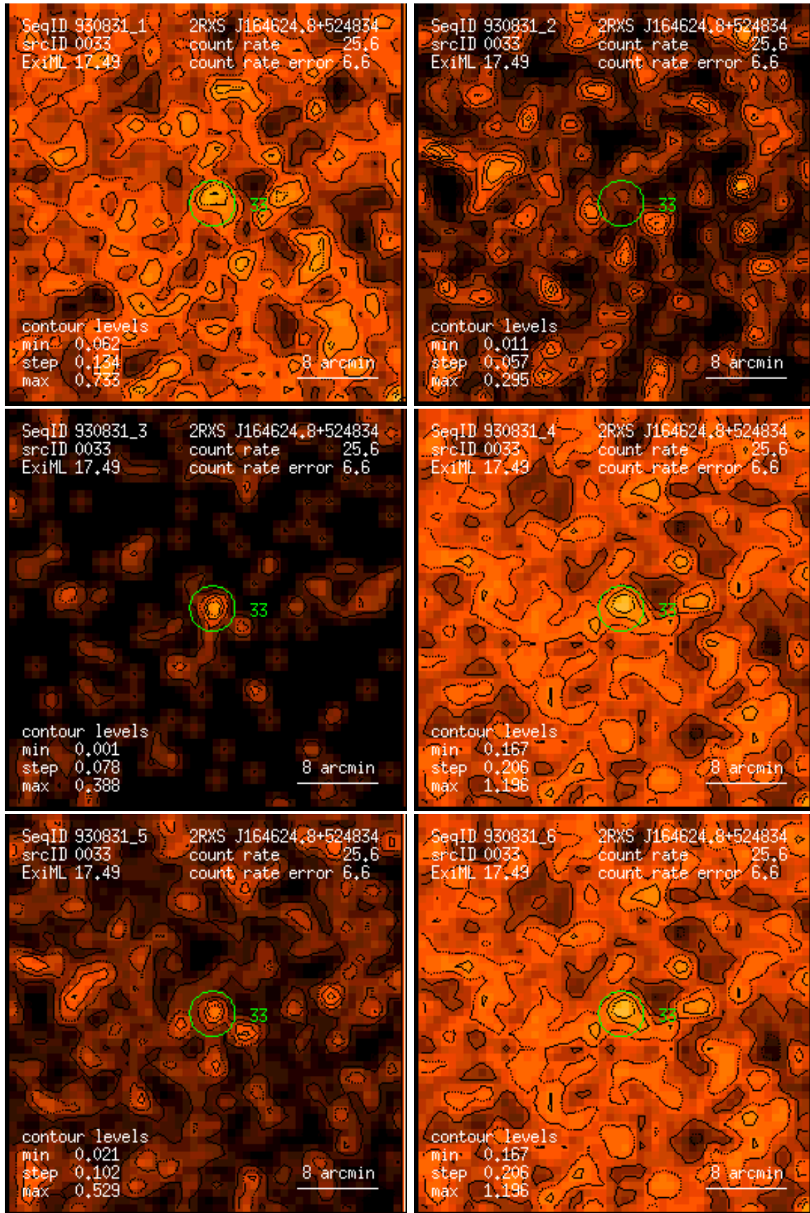
Figure 33: RASS 930831: detection 0033: band rate images, Gaussian filter: (1) PSPC channels 11 – 41, (2) 52 – 90, (3) 91 – 201, (4) 11 – 235, (5) 52 – 201, (6) 11 – 201. Broad band rates in counts/ks. Band rate contour levels in counts/ks/arcmin 2 .
