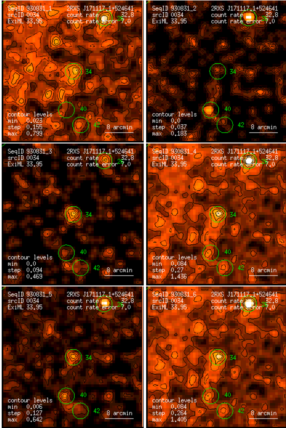
Figure 34: RASS 930831: detection 0034: band rate images, Gaussian filter: (1) PSPC channels 11 – 41, (2) 52 – 90, (3) 91 – 201, (4) 11 – 235, (5) 52 – 201, (6) 11 – 201. Broad band rates in counts/ks. Band rate contour levels in counts/ks/arcmin 2 .
