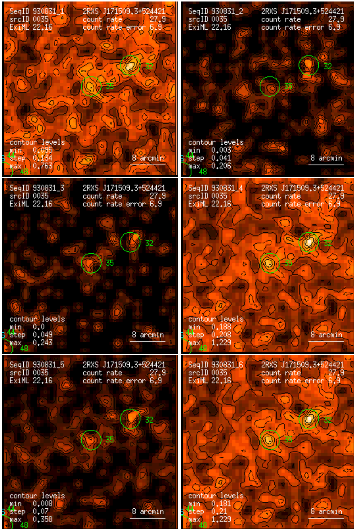
Figure 35: RASS 930831: detection 0035: band rate images, Gaussian filter: (1) PSPC channels 11 – 41, (2) 52 – 90, (3) 91 – 201, (4) 11 – 235, (5) 52 – 201, (6) 11 – 201. Broad band rates in counts/ks. Band rate contour levels in counts/ks/arcmin 2 .
