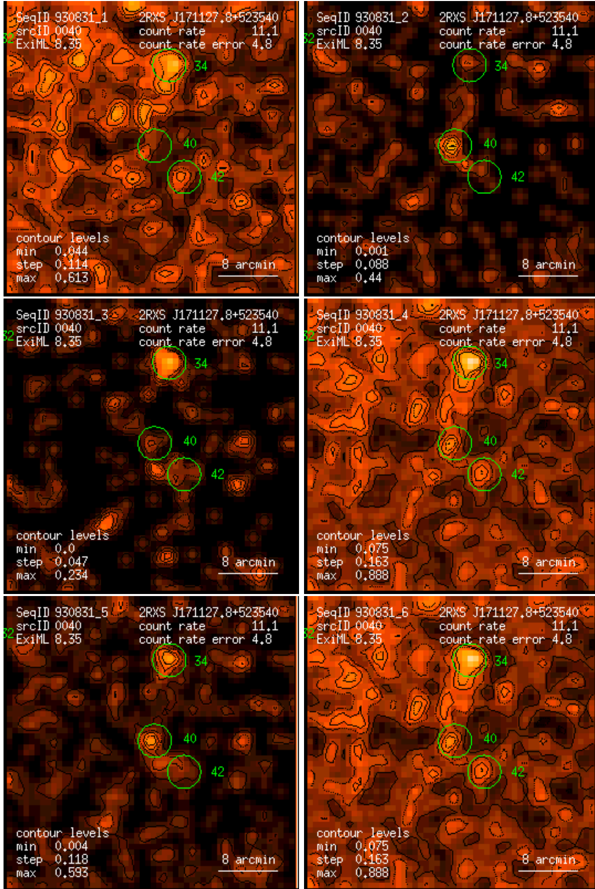
Figure 40: RASS 930831: detection 0040: band rate images, Gaussian filter: (1) PSPC channels 11 – 41, (2) 52 – 90, (3) 91 – 201, (4) 11 – 235, (5) 52 – 201, (6) 11 – 201. Broad band rates in counts/ks. Band rate contour levels in counts/ks/arcmin 2 .
