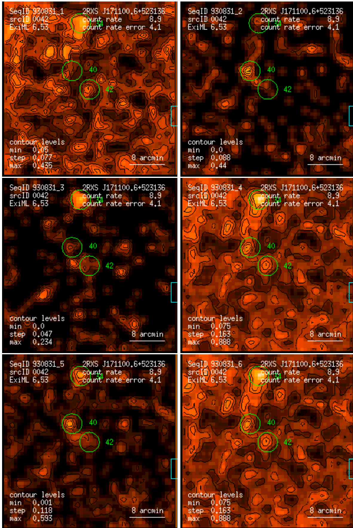
Figure 42: RASS 930831: detection 0042: band rate images, Gaussian filter: (1) PSPC channels 11 – 41, (2) 52 – 90, (3) 91 – 201, (4) 11 – 235, (5) 52 – 201, (6) 11 – 201. Broad band rates in counts/ks. Band rate contour levels in counts/ks/arcmin 2 .
