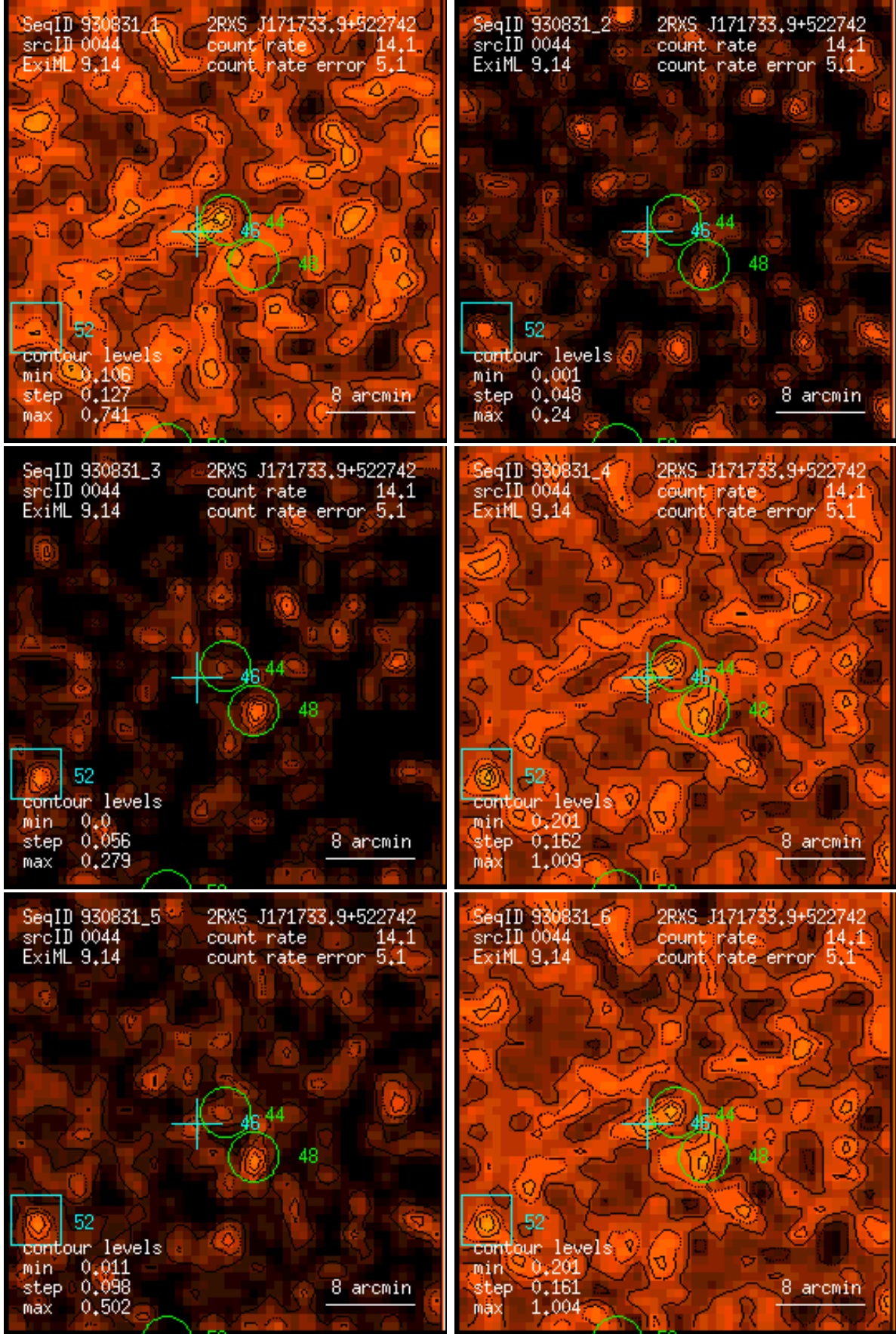
Figure 44: RASS 930831: detection 0044: band rate images, Gaussian filter: (1) PSPC channels 11 – 41, (2) 52 – 90, (3) 91 – 201, (4) 11 – 235, (5) 52 – 201, (6) 11 – 201. Broad band rates in counts/ks. Band rate contour levels in counts/ks/arcmin 2 .
