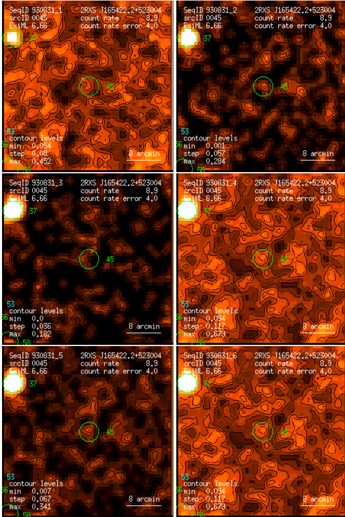
Figure 45: RASS 930831: detection 0045: band rate images, Gaussian filter: (1) PSPC channels 11 – 41, (2) 52 – 90, (3) 91 – 201, (4) 11 – 235, (5) 52 – 201, (6) 11 – 201. Broad band rates in counts/ks. Band rate contour levels in counts/ks/arcmin 2 .
