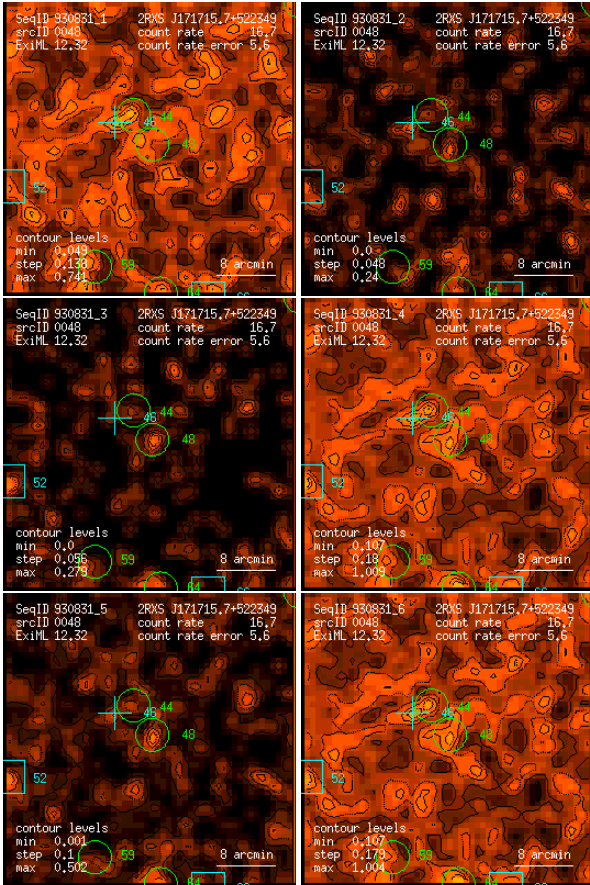
Figure 48: RASS 930831: detection 0048: band rate images, Gaussian filter: (1) PSPC channels 11 – 41, (2) 52 – 90, (3) 91 – 201, (4) 11 – 235, (5) 52 – 201, (6) 11 – 201. Broad band rates in counts/ks. Band rate contour levels in counts/ks/arcmin 2 .
