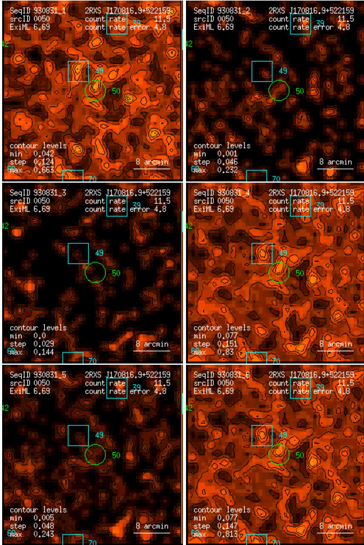
Figure 50: RASS 930831: detection 0050: band rate images, Gaussian filter: (1) PSPC channels 11 – 41, (2) 52 – 90, (3) 91 – 201, (4) 11 – 235, (5) 52 – 201, (6) 11 – 201. Broad band rates in counts/ks. Band rate contour levels in counts/ks/arcmin 2 .
