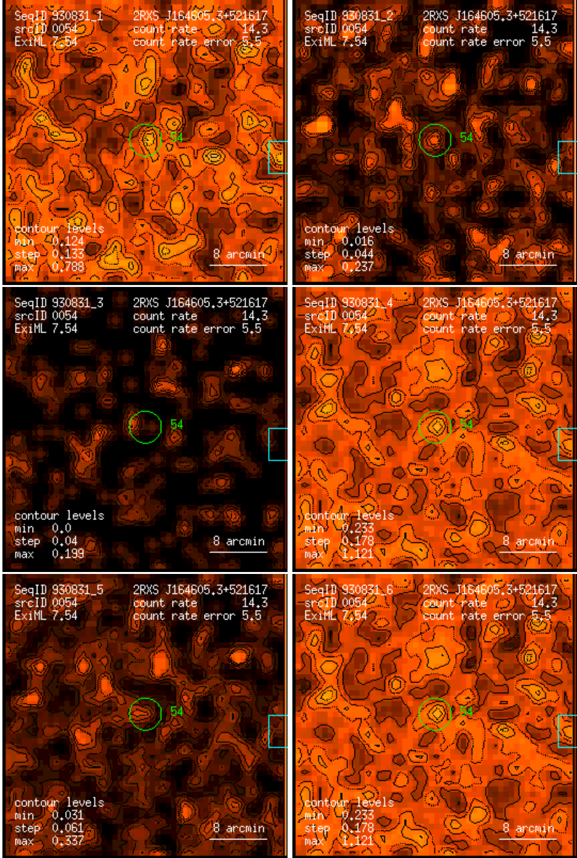
Figure 54: RASS 930831: detection 0054: band rate images, Gaussian filter: (1) PSPC channels 11 – 41, (2) 52 – 90, (3) 91 – 201, (4) 11 – 235, (5) 52 – 201, (6) 11 – 201. Broad band rates in counts/ks. Band rate contour levels in counts/ks/arcmin 2 .
