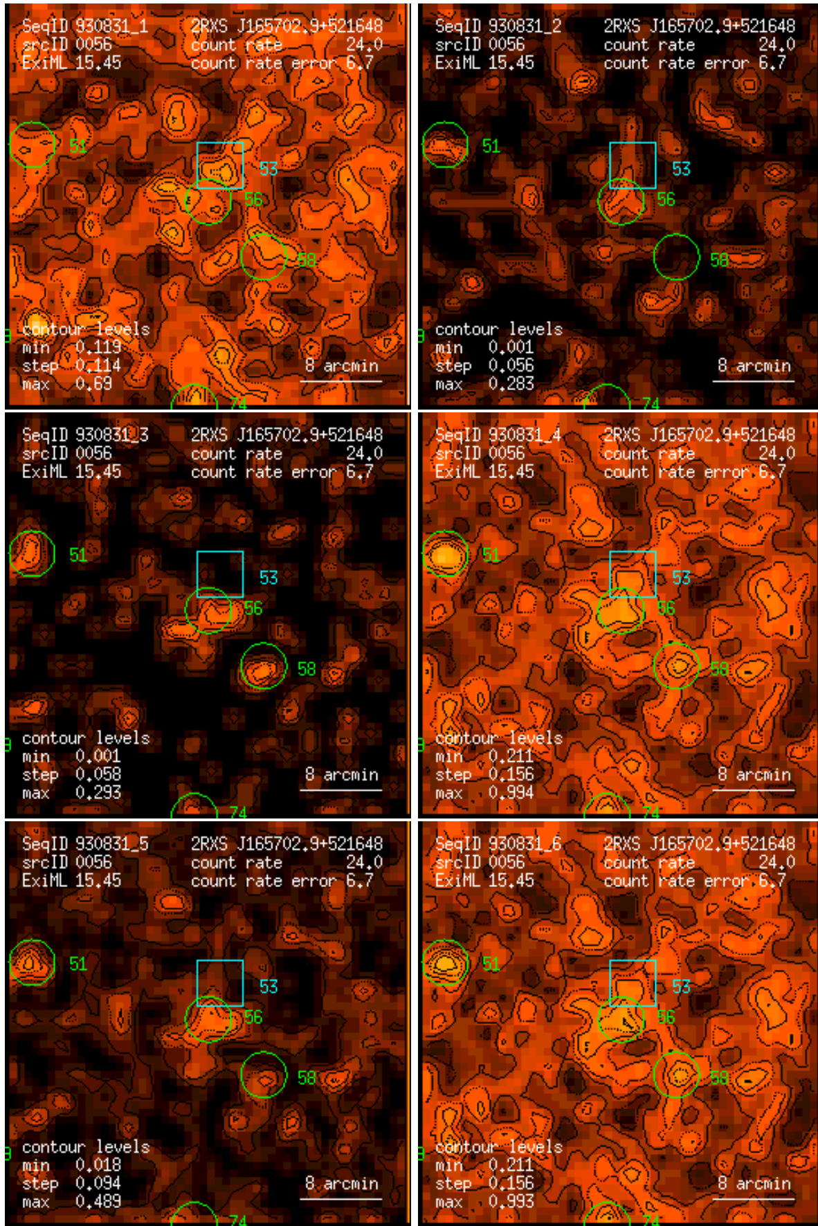
Figure 56: RASS 930831: detection 0056: band rate images, Gaussian filter: (1) PSPC channels 11 – 41, (2) 52 – 90, (3) 91 – 201, (4) 11 – 235, (5) 52 – 201, (6) 11 – 201. Broad band rates in counts/ks. Band rate contour levels in counts/ks/arcmin 2 .
