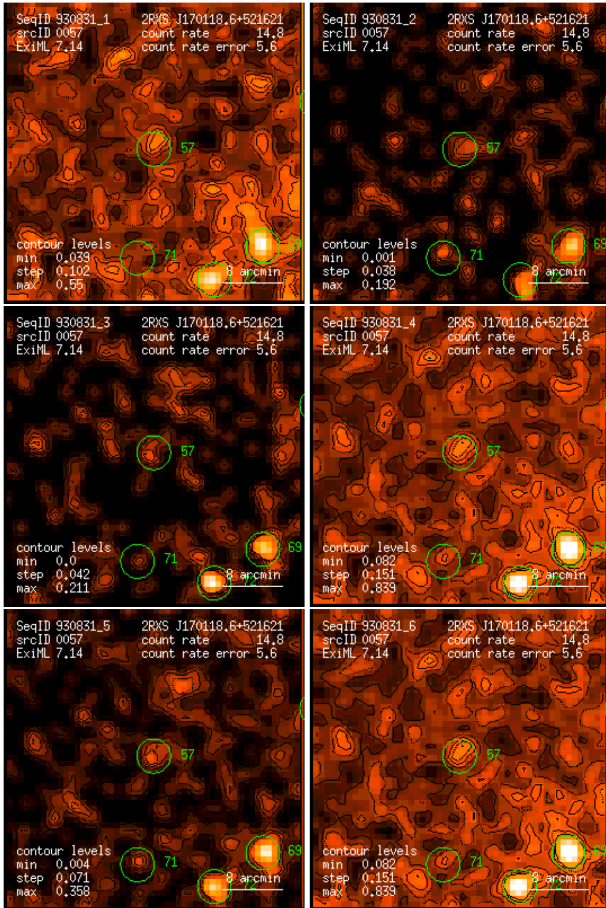
Figure 57: RASS 930831: detection 0057: band rate images, Gaussian filter: (1) PSPC channels 11 – 41, (2) 52 – 90, (3) 91 – 201, (4) 11 – 235, (5) 52 – 201, (6) 11 – 201. Broad band rates in counts/ks. Band rate contour levels in counts/ks/arcmin 2 .
