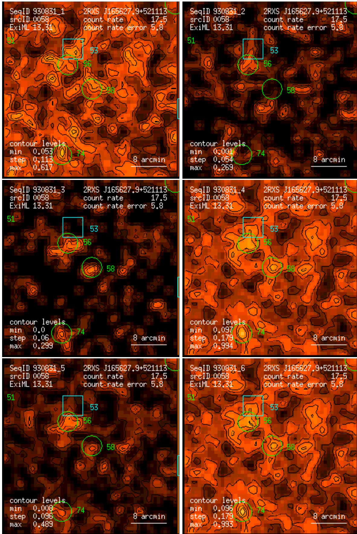
Figure 58: RASS 930831: detection 0058: band rate images, Gaussian filter: (1) PSPC channels 11 – 41, (2) 52 – 90, (3) 91 – 201, (4) 11 – 235, (5) 52 – 201, (6) 11 – 201. Broad band rates in counts/ks. Band rate contour levels in counts/ks/arcmin 2 .
