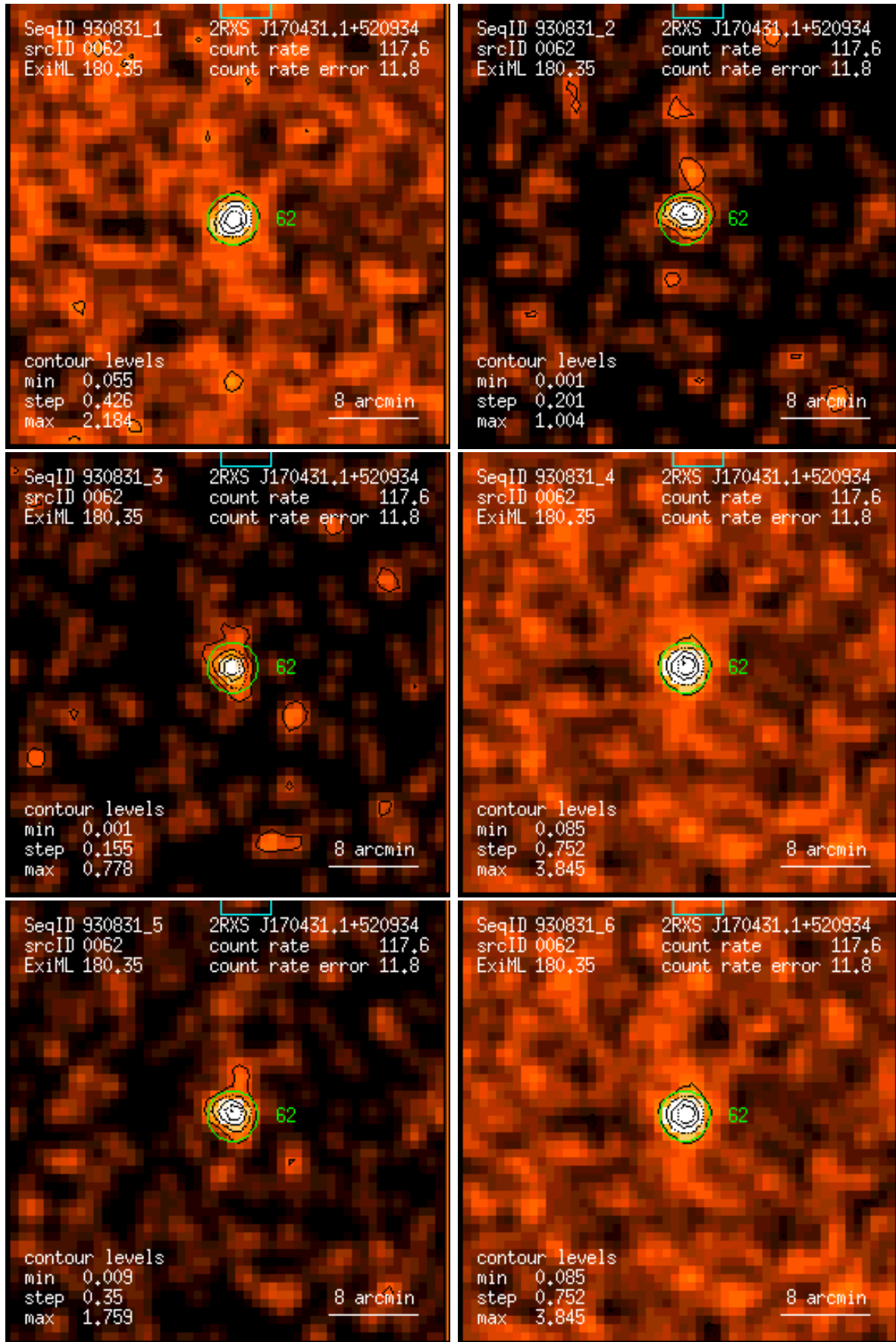
Figure 62: RASS 930831: detection 0062: band rate images, Gaussian filter: (1) PSPC channels 11 – 41, (2) 52 – 90, (3) 91 – 201, (4) 11 – 235, (5) 52 – 201, (6) 11 – 201. Broad band rates in counts/ks. Band rate contour levels in counts/ks/arcmin 2 .
