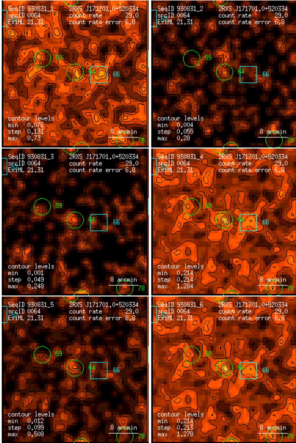
Figure 64: RASS 930831: detection 0064: band rate images, Gaussian filter: (1) PSPC channels 11 – 41, (2) 52 – 90, (3) 91 – 201, (4) 11 – 235, (5) 52 – 201, (6) 11 – 201. Broad band rates in counts/ks. Band rate contour levels in counts/ks/arcmin 2 .
