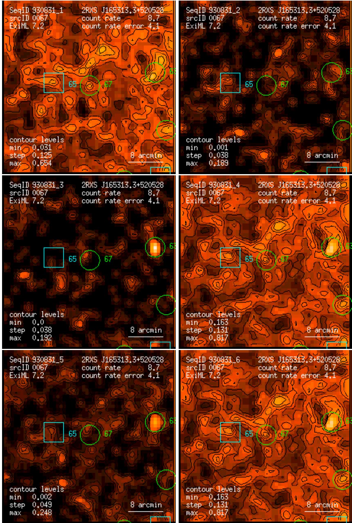
Figure 67: RASS 930831: detection 0067: band rate images, Gaussian filter: (1) PSPC channels 11 – 41, (2) 52 – 90, (3) 91 – 201, (4) 11 – 235, (5) 52 – 201, (6) 11 – 201. Broad band rates in counts/ks. Band rate contour levels in counts/ks/arcmin 2 .
