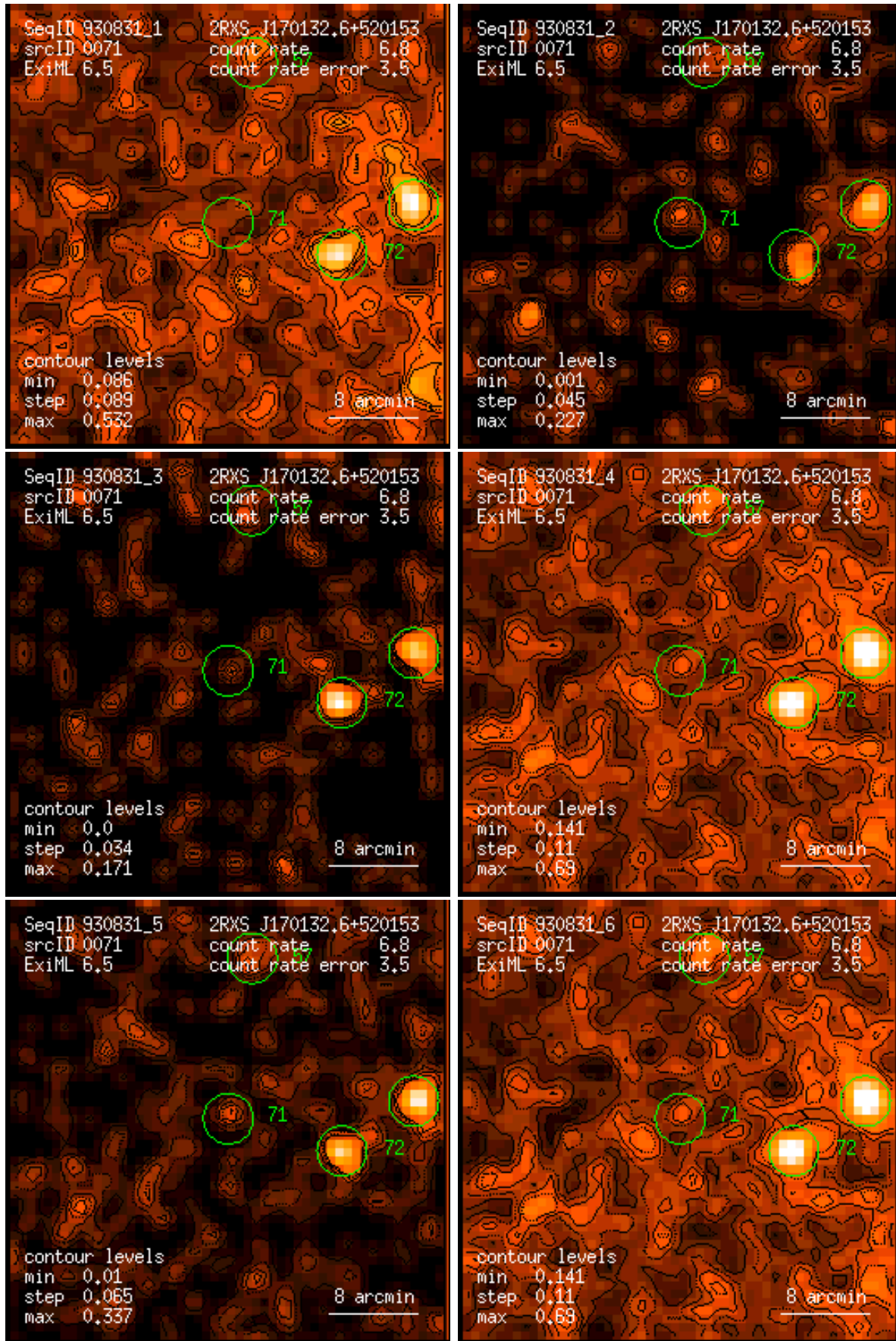
Figure 71: RASS 930831: detection 0071: band rate images, Gaussian filter: (1) PSPC channels 11 – 41, (2) 52 – 90, (3) 91 – 201, (4) 11 – 235, (5) 52 – 201, (6) 11 – 201. Broad band rates in counts/ks. Band rate contour levels in counts/ks/arcmin 2 .
