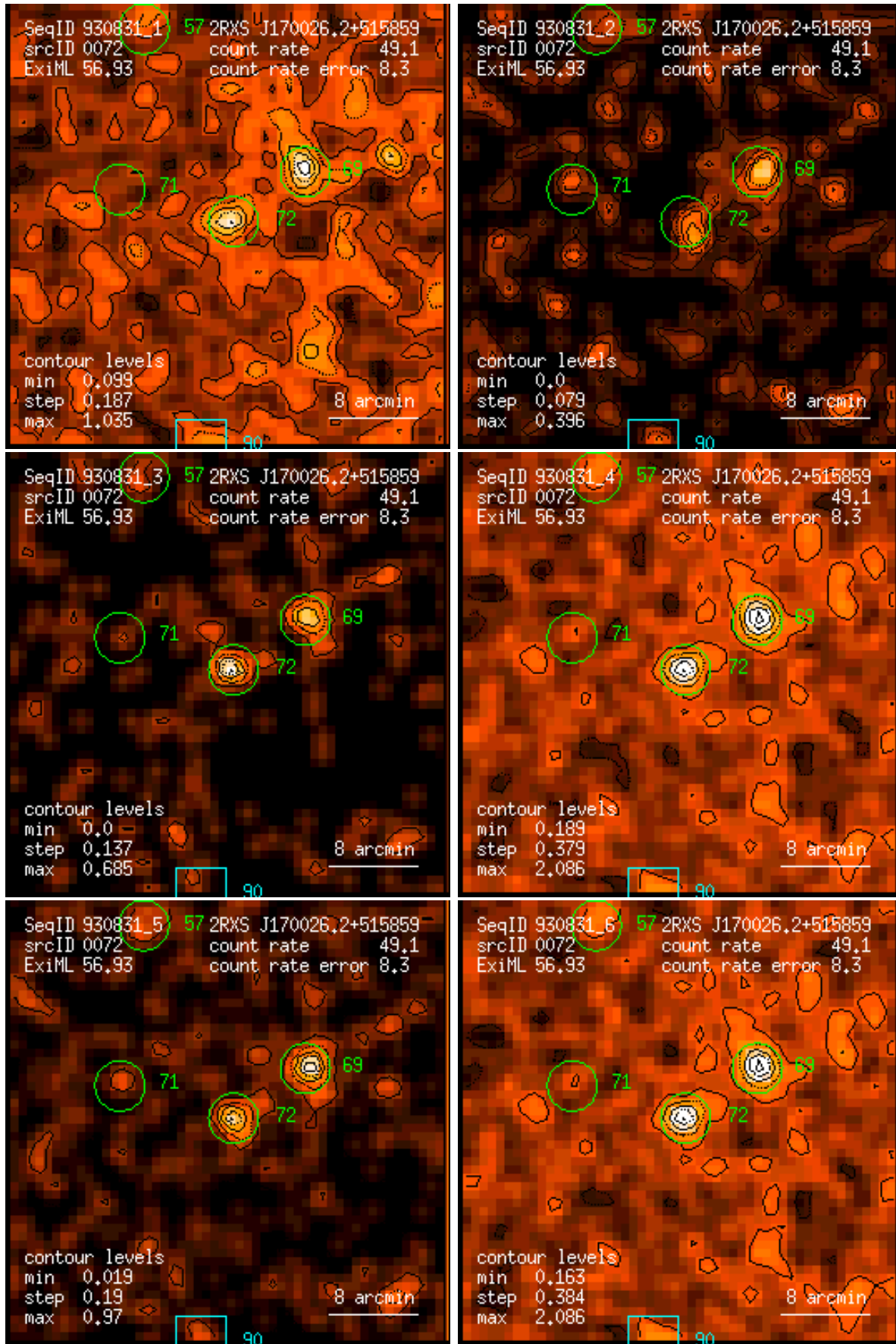
Figure 72: RASS 930831: detection 0072: band rate images, Gaussian filter: (1) PSPC channels 11 – 41, (2) 52 – 90, (3) 91 – 201, (4) 11 – 235, (5) 52 – 201, (6) 11 – 201. Broad band rates in counts/ks. Band rate contour levels in counts/ks/arcmin 2 .
