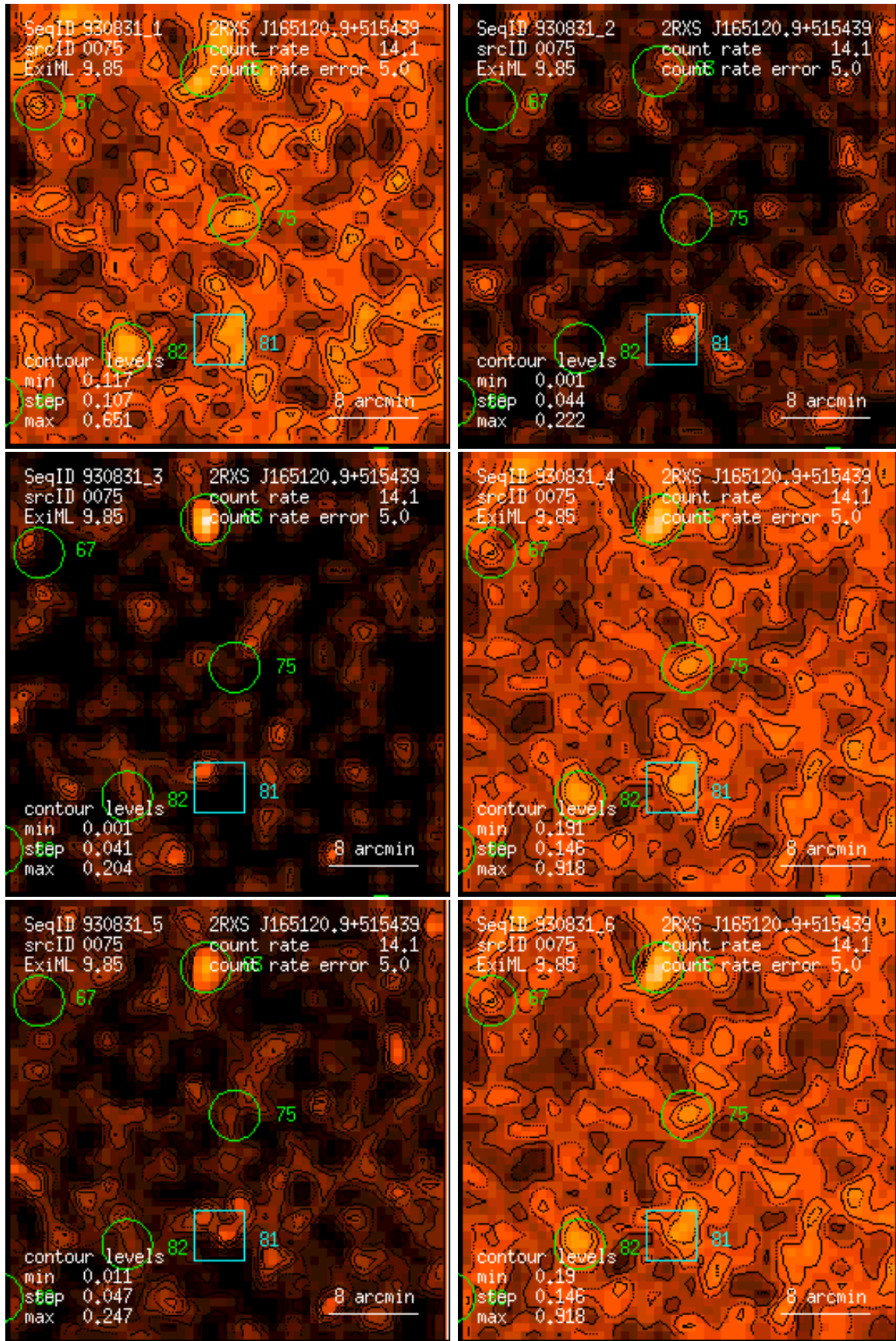
Figure 75: RASS 930831: detection 0075: band rate images, Gaussian filter: (1) PSPC channels 11 – 41, (2) 52 – 90, (3) 91 – 201, (4) 11 – 235, (5) 52 – 201, (6) 11 – 201. Broad band rates in counts/ks. Band rate contour levels in counts/ks/arcmin 2 .
