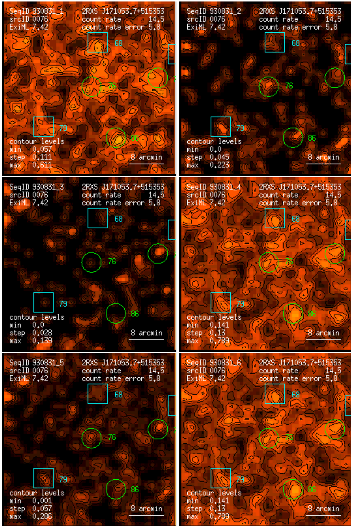
Figure 76: RASS 930831: detection 0076: band rate images, Gaussian filter: (1) PSPC channels 11 – 41, (2) 52 – 90, (3) 91 – 201, (4) 11 – 235, (5) 52 – 201, (6) 11 – 201. Broad band rates in counts/ks. Band rate contour levels in counts/ks/arcmin 2 .
