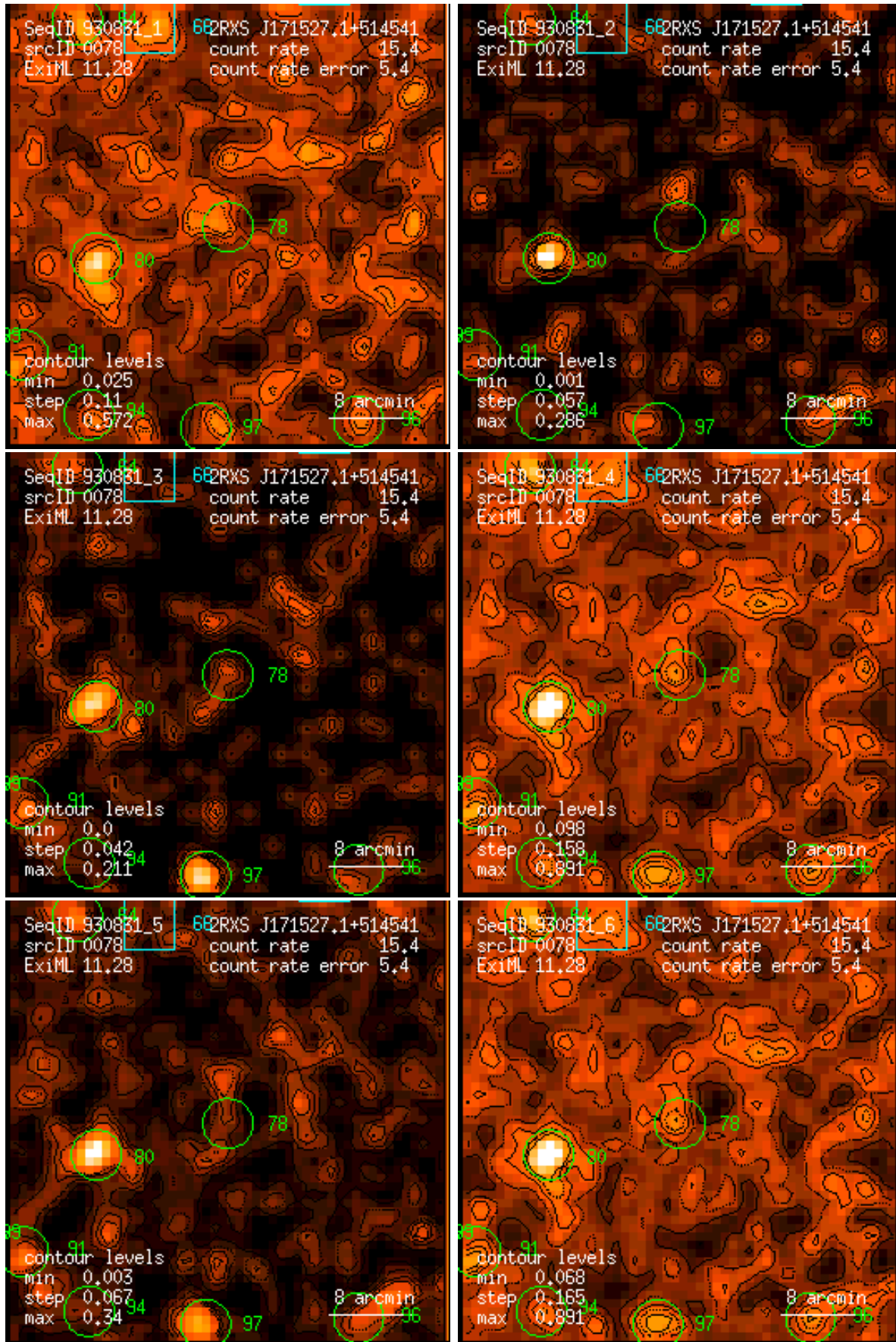
Figure 78: RASS 930831: detection 0078: band rate images, Gaussian filter: (1) PSPC channels 11 – 41, (2) 52 – 90, (3) 91 – 201, (4) 11 – 235, (5) 52 – 201, (6) 11 – 201. Broad band rates in counts/ks. Band rate contour levels in counts/ks/arcmin 2 .
