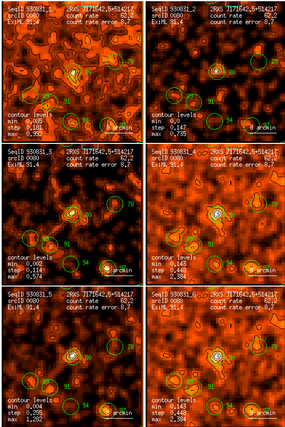
Figure 80: RASS 930831: detection 0080: band rate images, Gaussian filter: (1) PSPC channels 11 – 41, (2) 52 – 90, (3) 91 – 201, (4) 11 – 235, (5) 52 – 201, (6) 11 – 201. Broad band rates in counts/ks. Band rate contour levels in counts/ks/arcmin 2 .
