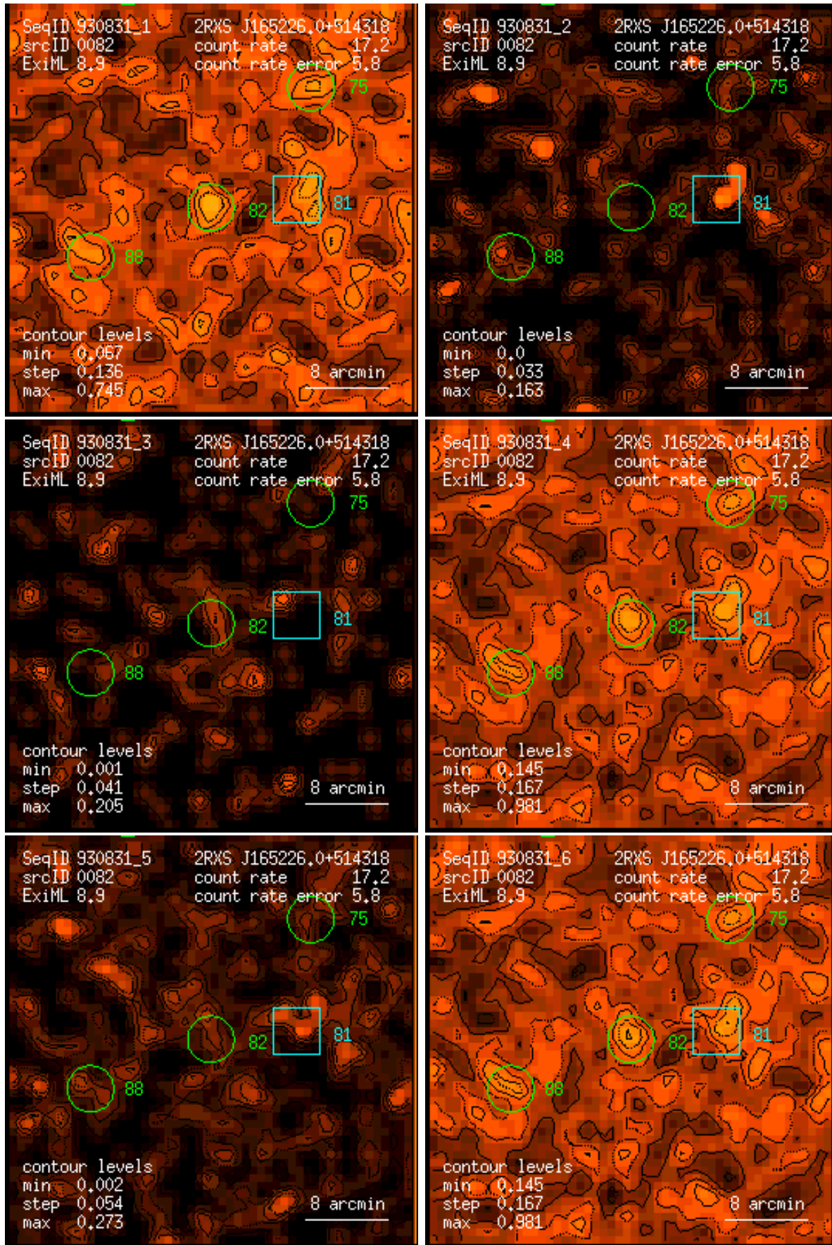
Figure 82: RASS 930831: detection 0082: band rate images, Gaussian filter: (1) PSPC channels 11 – 41, (2) 52 – 90, (3) 91 – 201, (4) 11 – 235, (5) 52 – 201, (6) 11 – 201. Broad band rates in counts/ks. Band rate contour levels in counts/ks/arcmin 2 .
