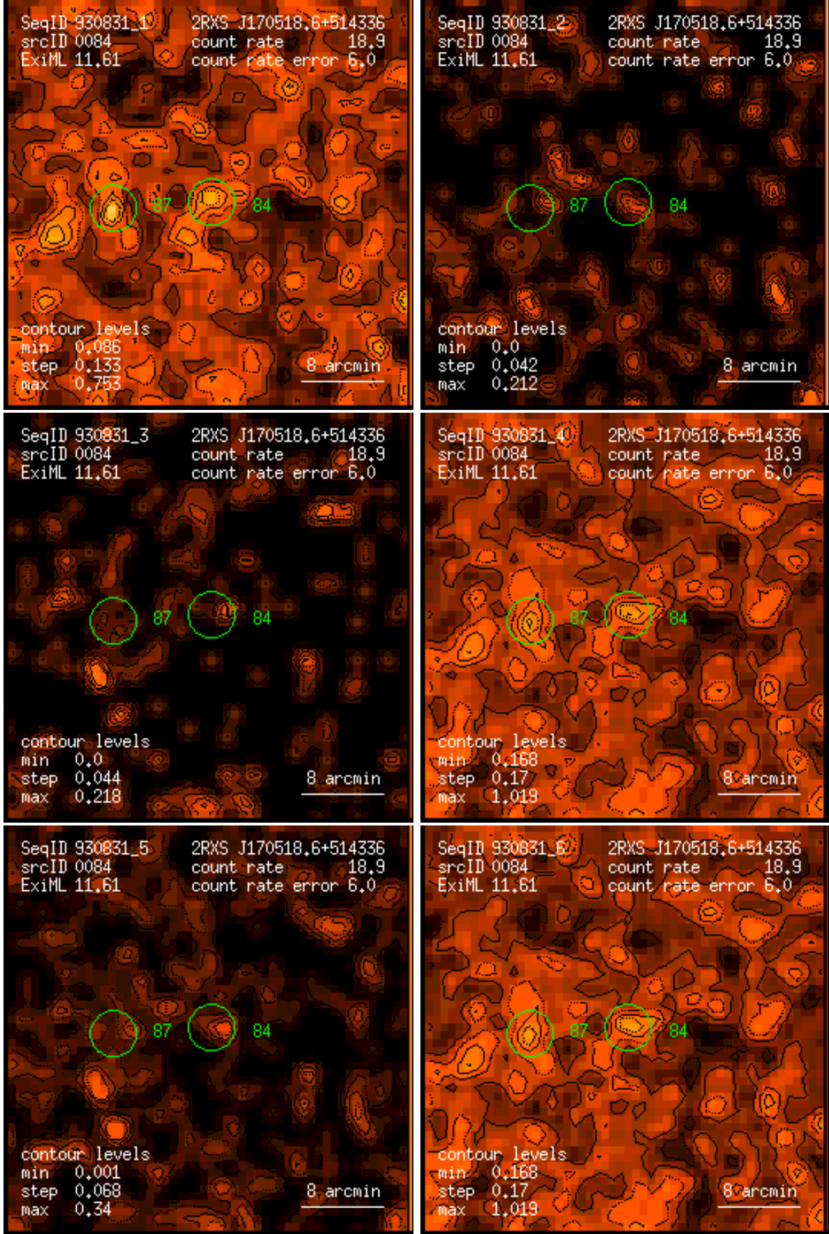
Figure 84: RASS 930831: detection 0084: band rate images, Gaussian filter: (1) PSPC channels 11 – 41, (2) 52 – 90, (3) 91 – 201, (4) 11 – 235, (5) 52 – 201, (6) 11 – 201. Broad band rates in counts/ks. Band rate contour levels in counts/ks/arcmin 2 .
