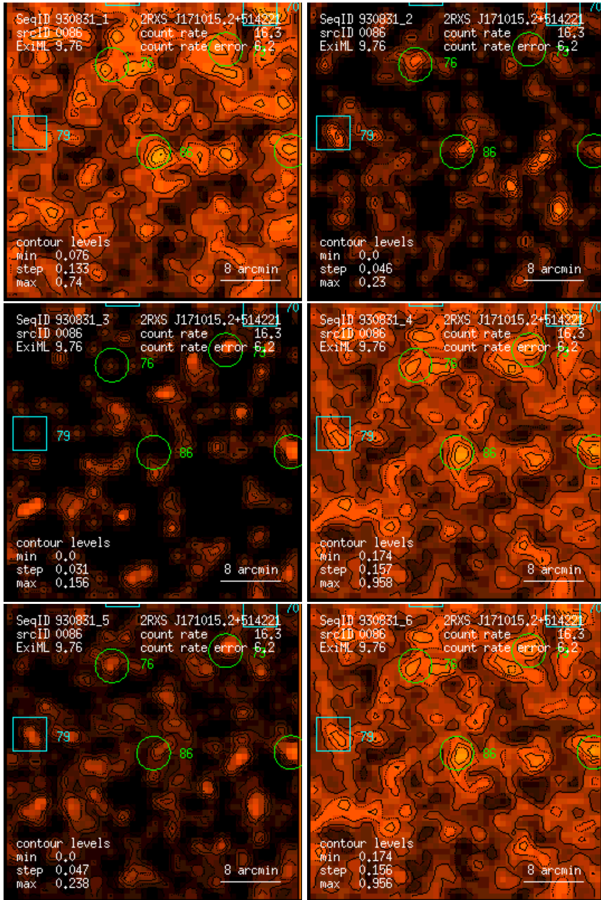
Figure 86: RASS 930831: detection 0086: band rate images, Gaussian filter: (1) PSPC channels 11 – 41, (2) 52 – 90, (3) 91 – 201, (4) 11 – 235, (5) 52 – 201, (6) 11 – 201. Broad band rates in counts/ks. Band rate contour levels in counts/ks/arcmin 2 .
