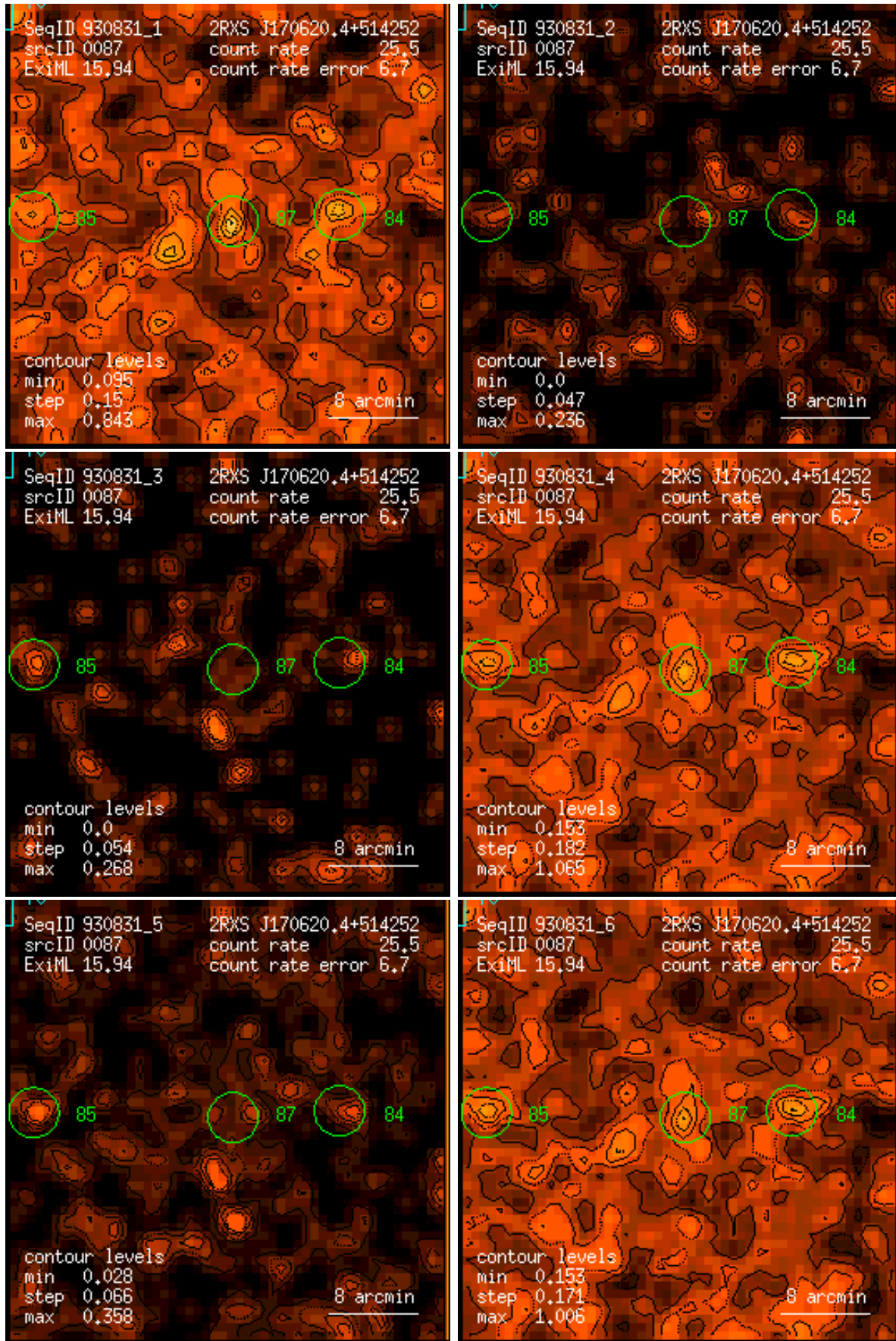
Figure 87: RASS 930831: detection 0087: band rate images, Gaussian filter: (1) PSPC channels 11 – 41, (2) 52 – 90, (3) 91 – 201, (4) 11 – 235, (5) 52 – 201, (6) 11 – 201. Broad band rates in counts/ks. Band rate contour levels in counts/ks/arcmin 2 .
