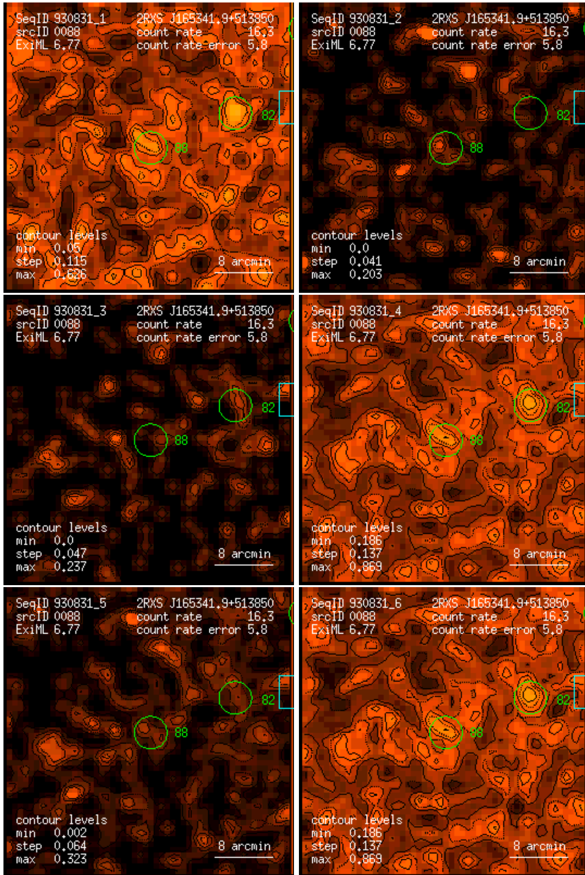
Figure 88: RASS 930831: detection 0088: band rate images, Gaussian filter: (1) PSPC channels 11 – 41, (2) 52 – 90, (3) 91 – 201, (4) 11 – 235, (5) 52 – 201, (6) 11 – 201. Broad band rates in counts/ks. Band rate contour levels in counts/ks/arcmin 2 .
