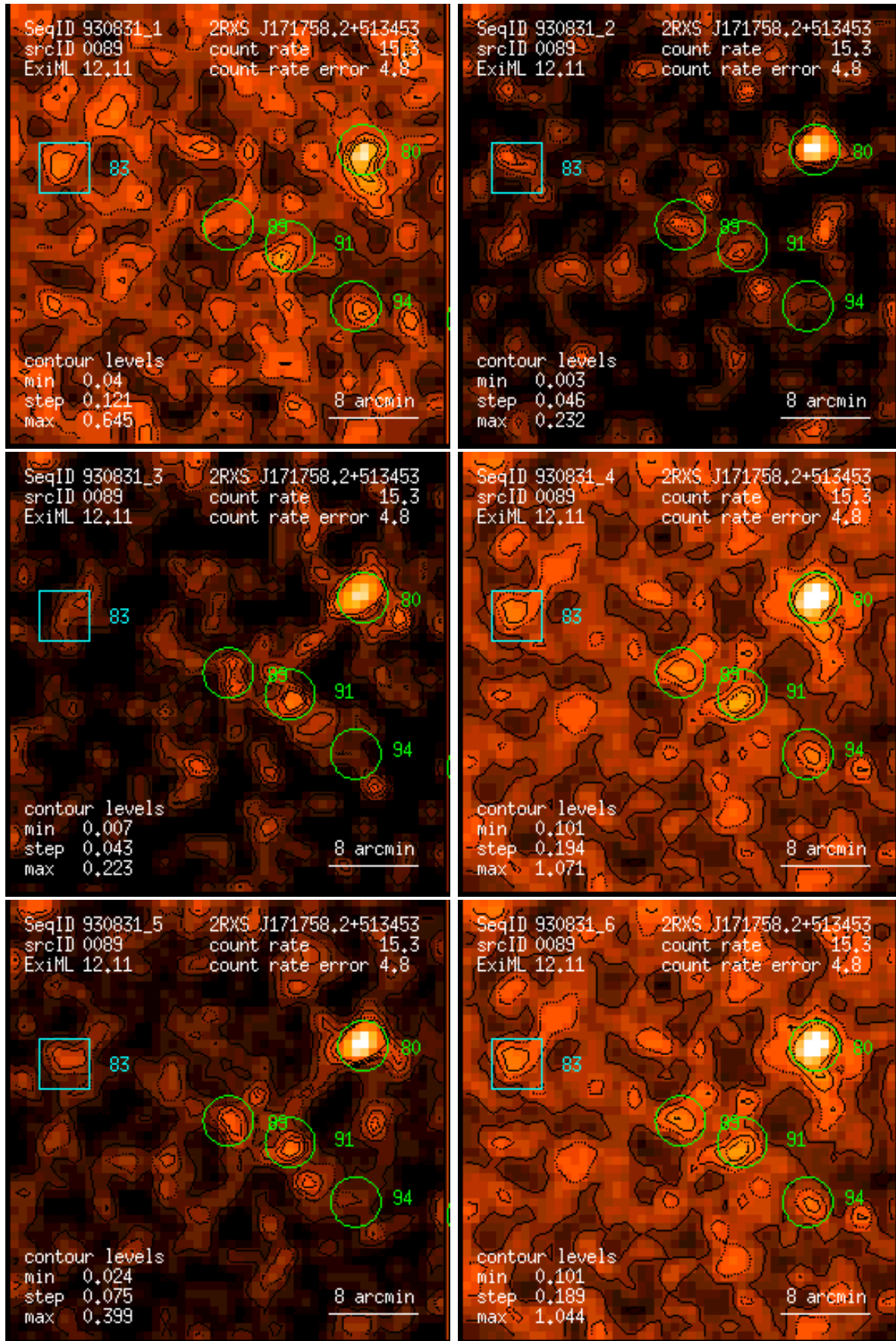
Figure 89: RASS 930831: detection 0089: band rate images, Gaussian filter: (1) PSPC channels 11 – 41, (2) 52 – 90, (3) 91 – 201, (4) 11 – 235, (5) 52 – 201, (6) 11 – 201. Broad band rates in counts/ks. Band rate contour levels in counts/ks/arcmin 2 .
