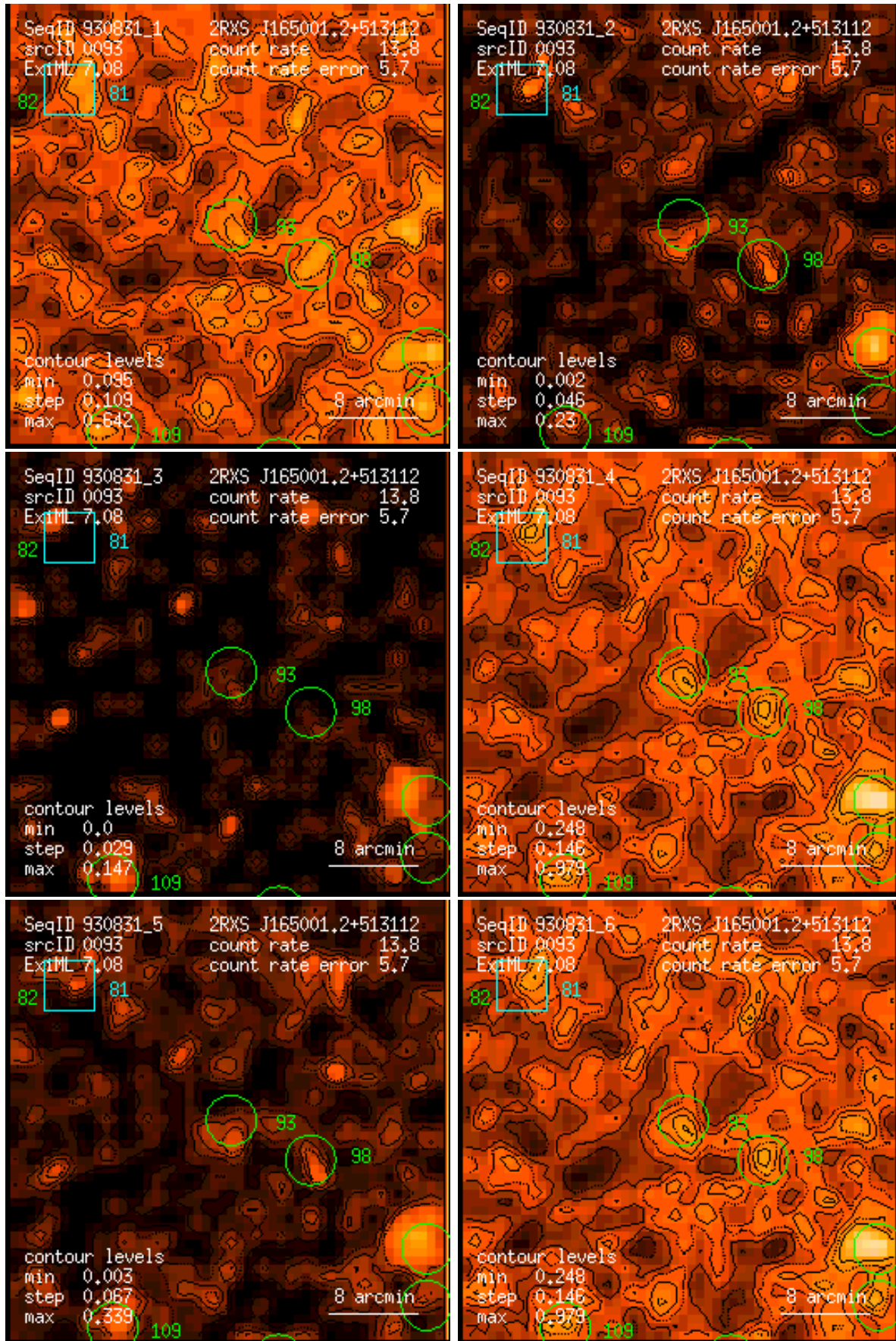
Figure 93: RASS 930831: detection 0093: band rate images, Gaussian filter: (1) PSPC channels 11 – 41, (2) 52 – 90, (3) 91 – 201, (4) 11 – 235, (5) 52 – 201, (6) 11 – 201. Broad band rates in counts/ks. Band rate contour levels in counts/ks/arcmin 2 .
