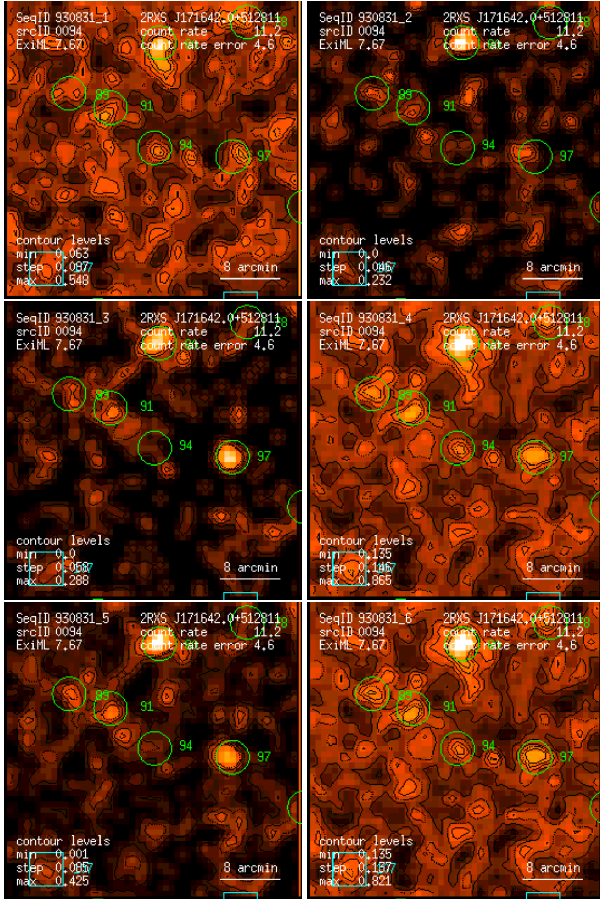
Figure 94: RASS 930831: detection 0094: band rate images, Gaussian filter: (1) PSPC channels 11 – 41, (2) 52 – 90, (3) 91 – 201, (4) 11 – 235, (5) 52 – 201, (6) 11 – 201. Broad band rates in counts/ks. Band rate contour levels in counts/ks/arcmin 2 .
