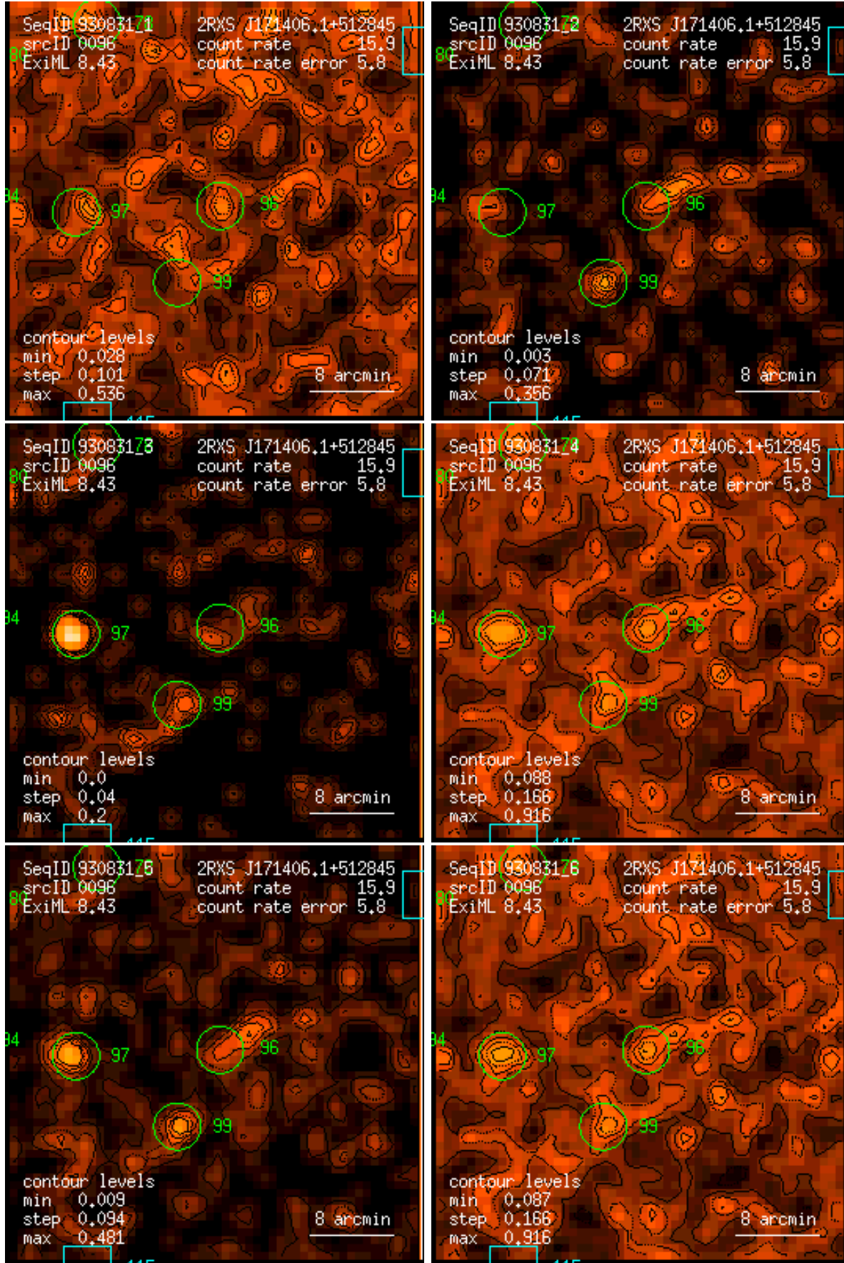
Figure 96: RASS 930831: detection 0096: band rate images, Gaussian filter: (1) PSPC channels 11 – 41, (2) 52 – 90, (3) 91 – 201, (4) 11 – 235, (5) 52 – 201, (6) 11 – 201. Broad band rates in counts/ks. Band rate contour levels in counts/ks/arcmin 2 .
