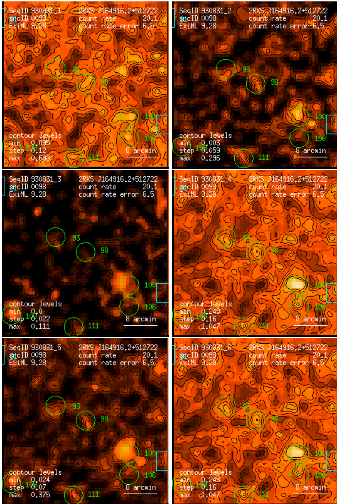
Figure 98: RASS 930831: detection 0098: band rate images, Gaussian filter: (1) PSPC channels 11 – 41, (2) 52 – 90, (3) 91 – 201, (4) 11 – 235, (5) 52 – 201, (6) 11 – 201. Broad band rates in counts/ks. Band rate contour levels in counts/ks/arcmin 2 .
