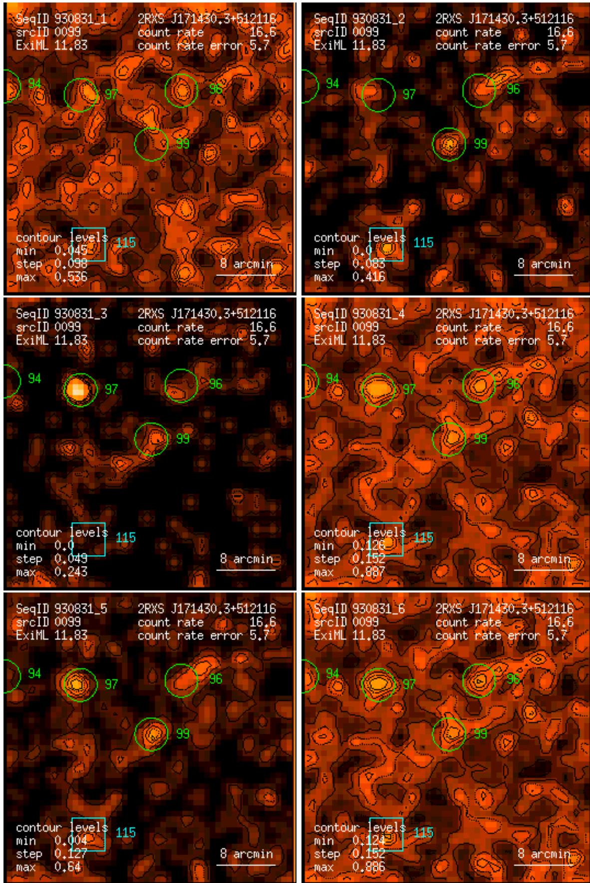
Figure 99: RASS 930831: detection 0099: band rate images, Gaussian filter: (1) PSPC channels 11 – 41, (2) 52 – 90, (3) 91 – 201, (4) 11 – 235, (5) 52 – 201, (6) 11 – 201. Broad band rates in counts/ks. Band rate contour levels in counts/ks/arcmin 2 .
