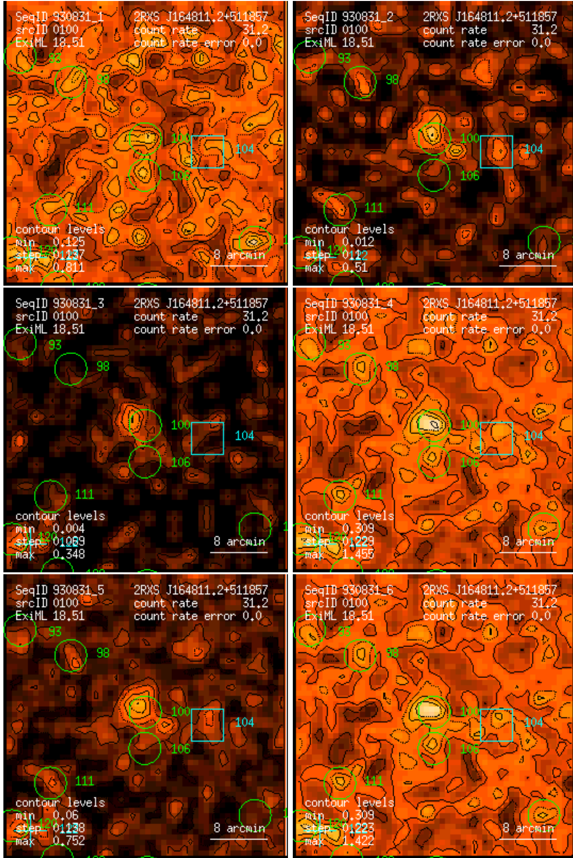
Figure 100: RASS 930831: detection 0100: band rate images, Gaussian filter: (1) PSPC channels 11 – 41, (2) 52 – 90, (3) 91 – 201, (4) 11 – 235, (5) 52 – 201, (6) 11 – 201. Broad band rates in counts/ks. Band rate contour levels in counts/ks/arcmin 2 .
