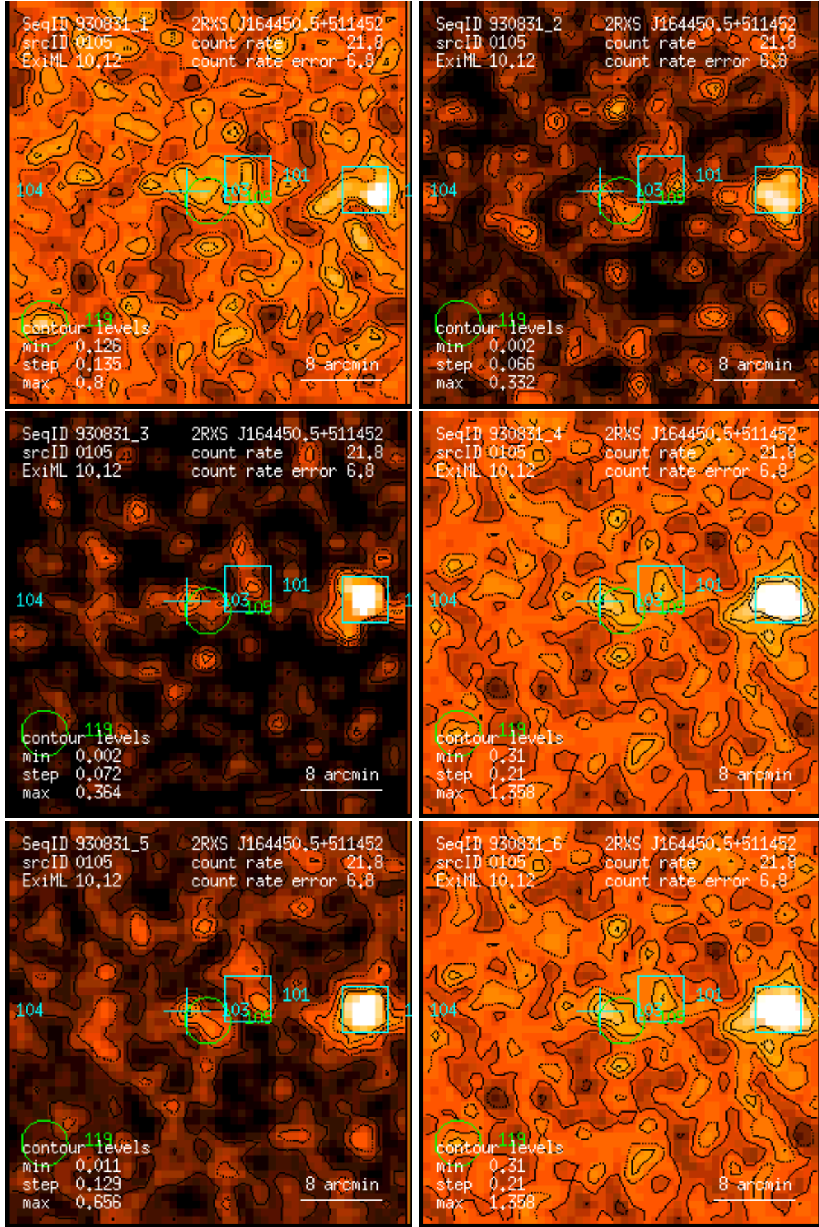
Figure 105: RASS 930831: detection 0105: band rate images, Gaussian filter: (1) PSPC channels 11 – 41, (2) 52 – 90, (3) 91 – 201, (4) 11 – 235, (5) 52 – 201, (6) 11 – 201. Broad band rates in counts/ks. Band rate contour levels in counts/ks/arcmin 2 .
