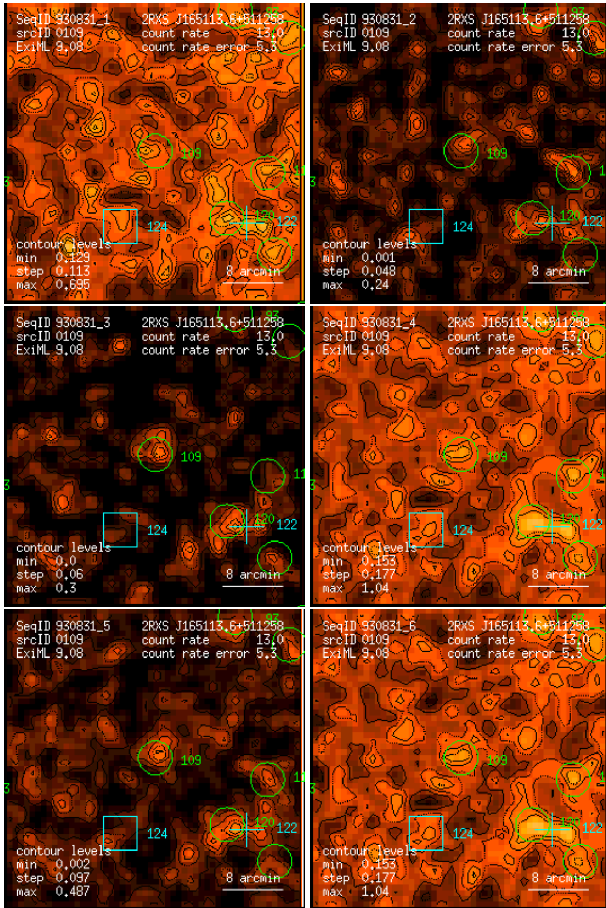
Figure 109: RASS 930831: detection 0109: band rate images, Gaussian filter: (1) PSPC channels 11 – 41, (2) 52 – 90, (3) 91 – 201, (4) 11 – 235, (5) 52 – 201, (6) 11 – 201. Broad band rates in counts/ks. Band rate contour levels in counts/ks/arcmin 2 .
