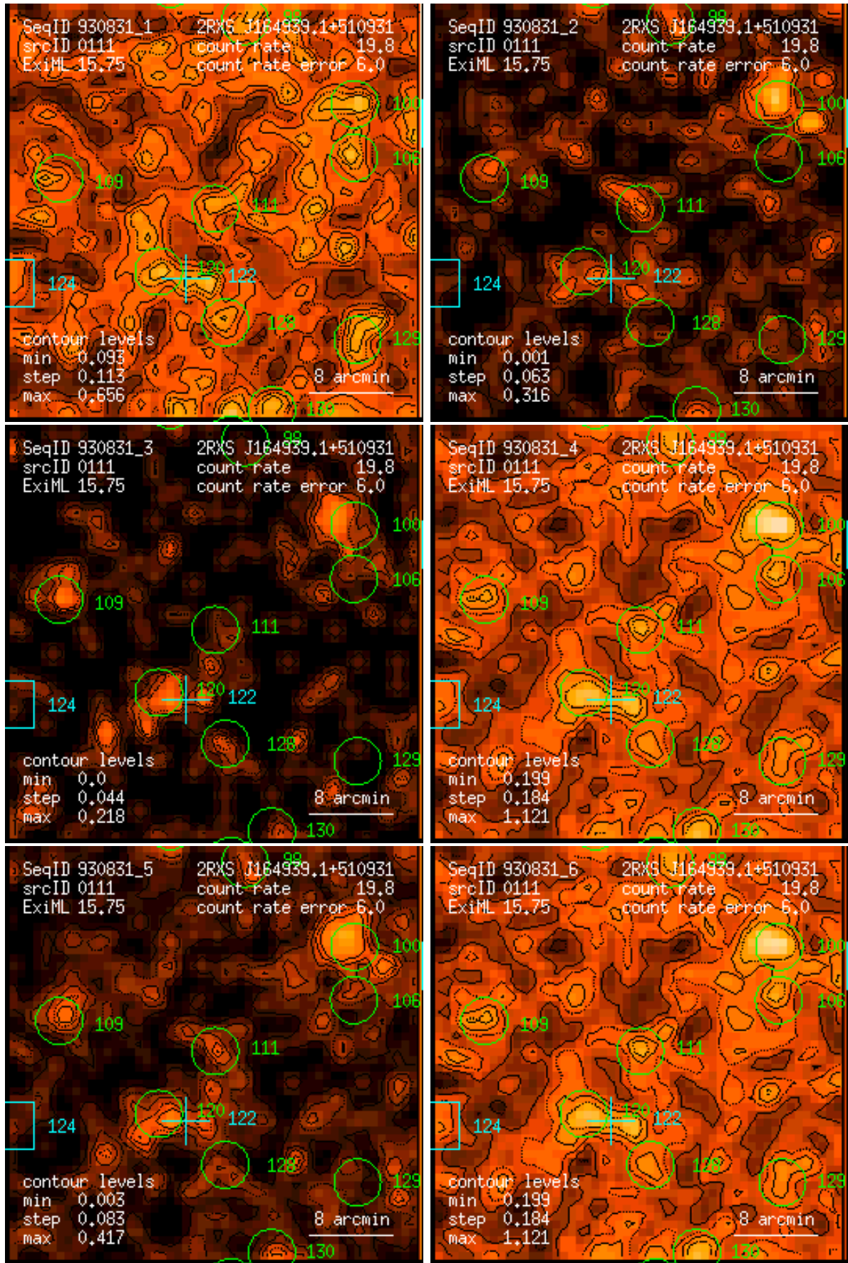
Figure 111: RASS 930831: detection 0111: band rate images, Gaussian filter: (1) PSPC channels 11 – 41, (2) 52 – 90, (3) 91 – 201, (4) 11 – 235, (5) 52 – 201, (6) 11 – 201. Broad band rates in counts/ks. Band rate contour levels in counts/ks/arcmin 2 .
