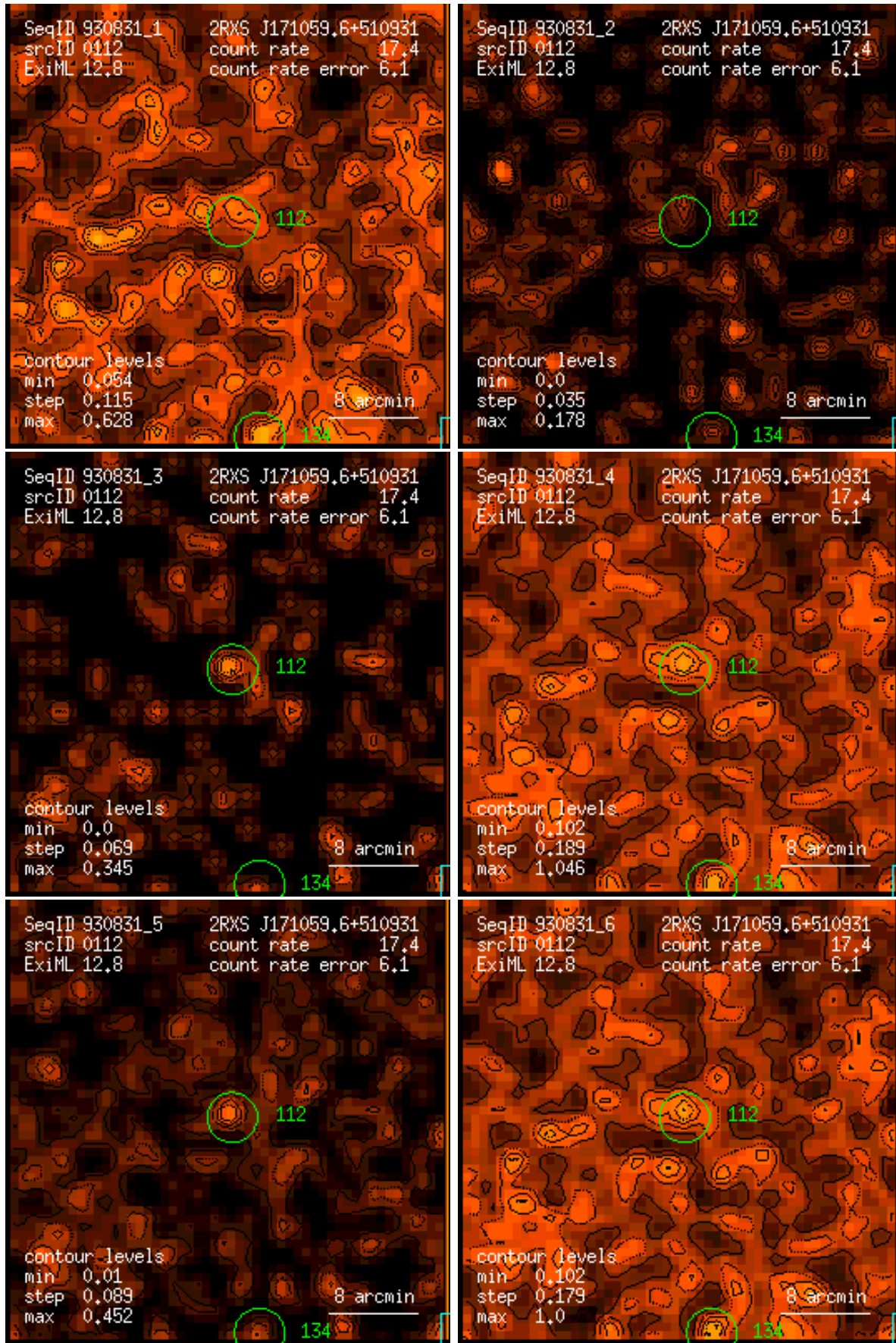
Figure 112: RASS 930831: detection 0112: band rate images, Gaussian filter: (1) PSPC channels 11 – 41, (2) 52 – 90, (3) 91 – 201, (4) 11 – 235, (5) 52 – 201, (6) 11 – 201. Broad band rates in counts/ks. Band rate contour levels in counts/ks/arcmin 2 .
