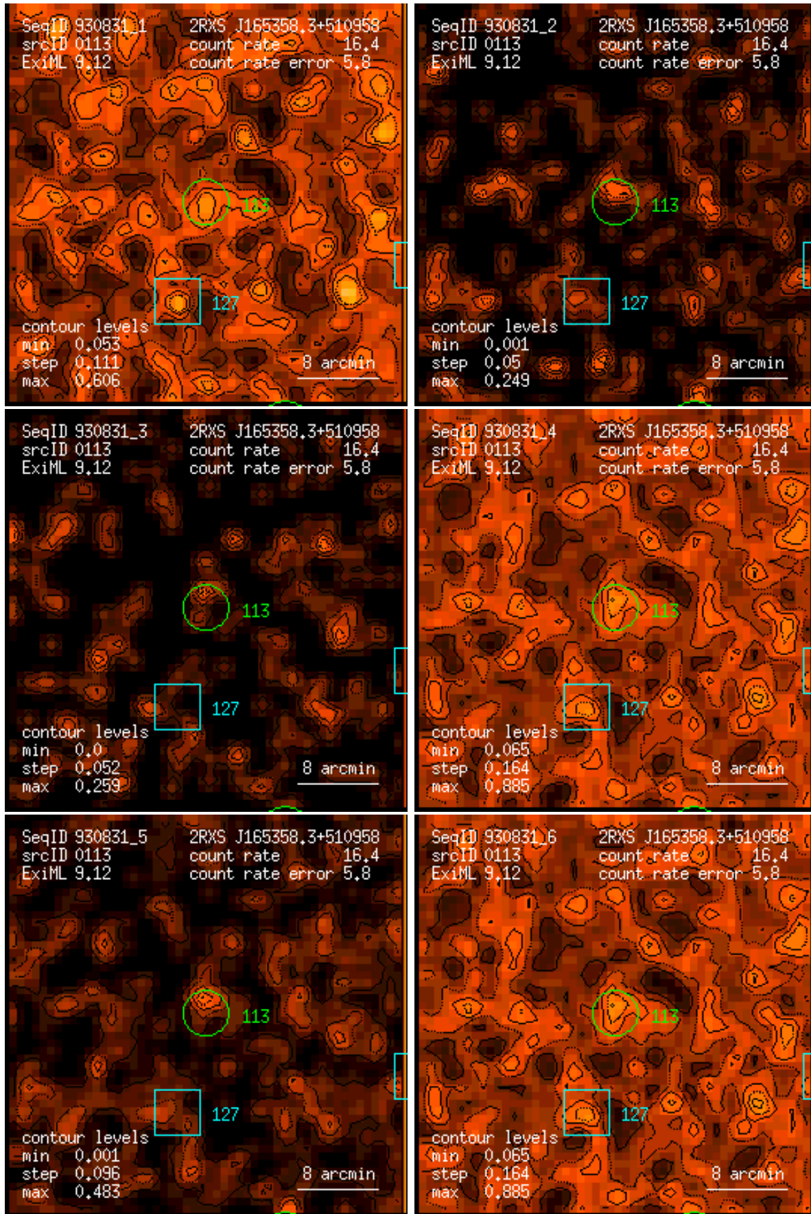
Figure 113: RASS 930831: detection 0113: band rate images, Gaussian filter: (1) PSPC channels 11 – 41, (2) 52 – 90, (3) 91 – 201, (4) 11 – 235, (5) 52 – 201, (6) 11 – 201. Broad band rates in counts/ks. Band rate contour levels in counts/ks/arcmin 2 .
