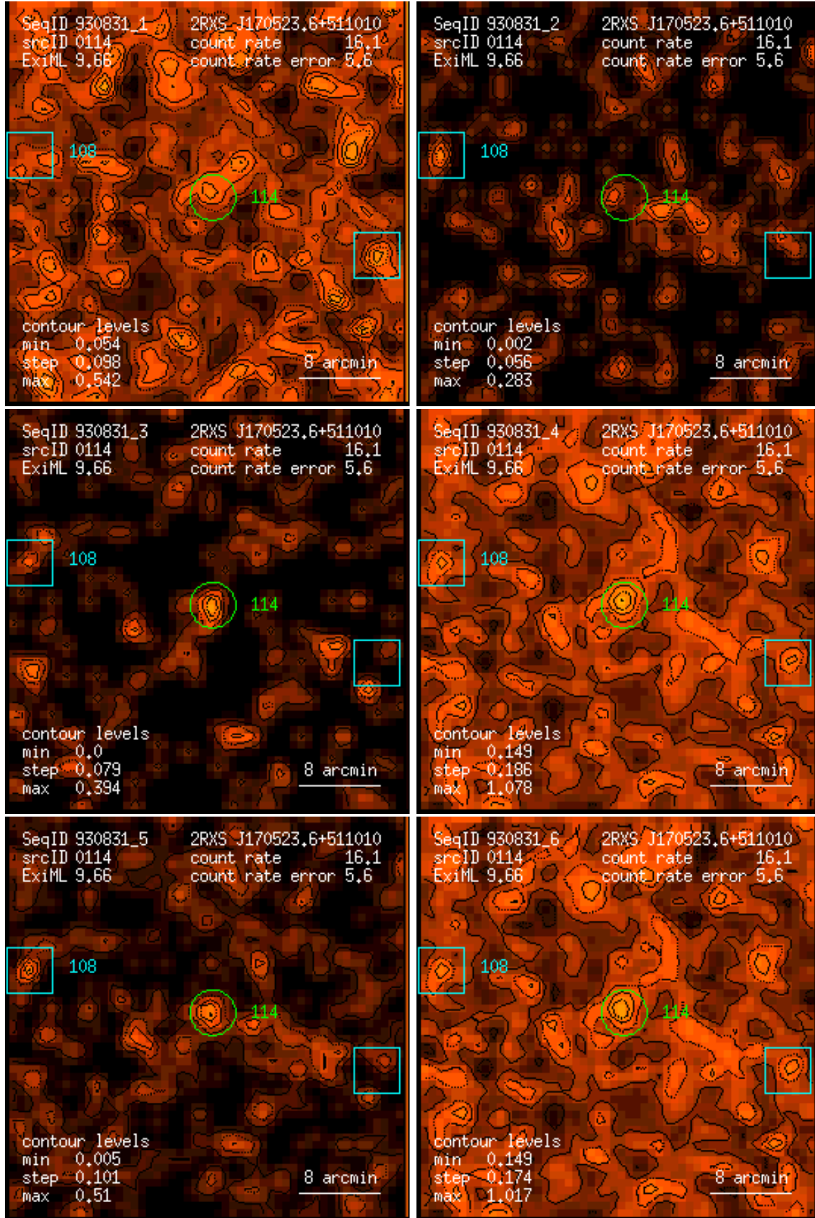
Figure 114: RASS 930831: detection 0114: band rate images, Gaussian filter: (1) PSPC channels 11 – 41, (2) 52 – 90, (3) 91 – 201, (4) 11 – 235, (5) 52 – 201, (6) 11 – 201. Broad band rates in counts/ks. Band rate contour levels in counts/ks/arcmin 2 .
