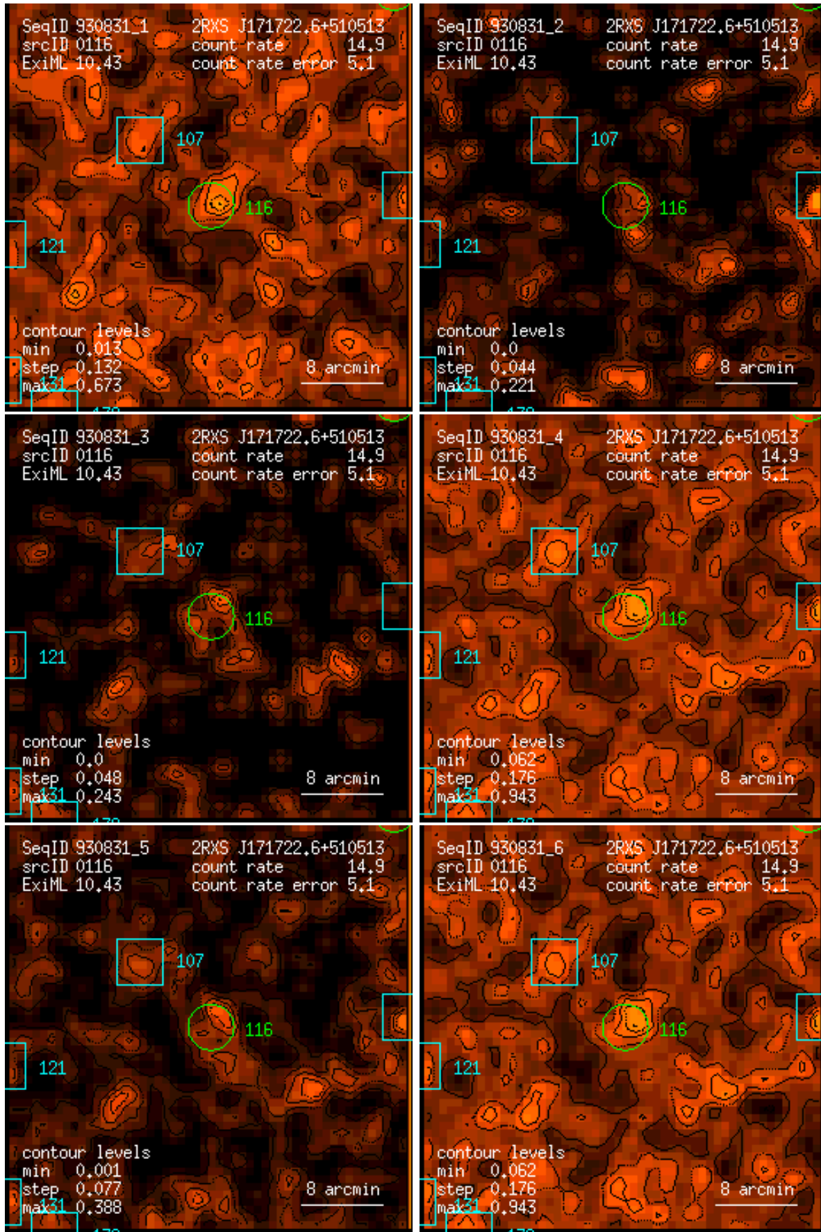
Figure 116: RASS 930831: detection 0116: band rate images, Gaussian filter: (1) PSPC channels 11 – 41, (2) 52 – 90, (3) 91 – 201, (4) 11 – 235, (5) 52 – 201, (6) 11 – 201. Broad band rates in counts/ks. Band rate contour levels in counts/ks/arcmin 2 .
