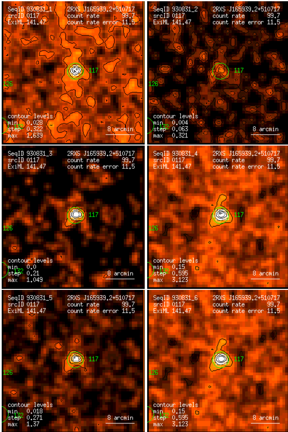
Figure 117: RASS 930831: detection 0117: band rate images, Gaussian filter: (1) PSPC channels 11 – 41, (2) 52 – 90, (3) 91 – 201, (4) 11 – 235, (5) 52 – 201, (6) 11 – 201. Broad band rates in counts/ks. Band rate contour levels in counts/ks/arcmin 2 .
