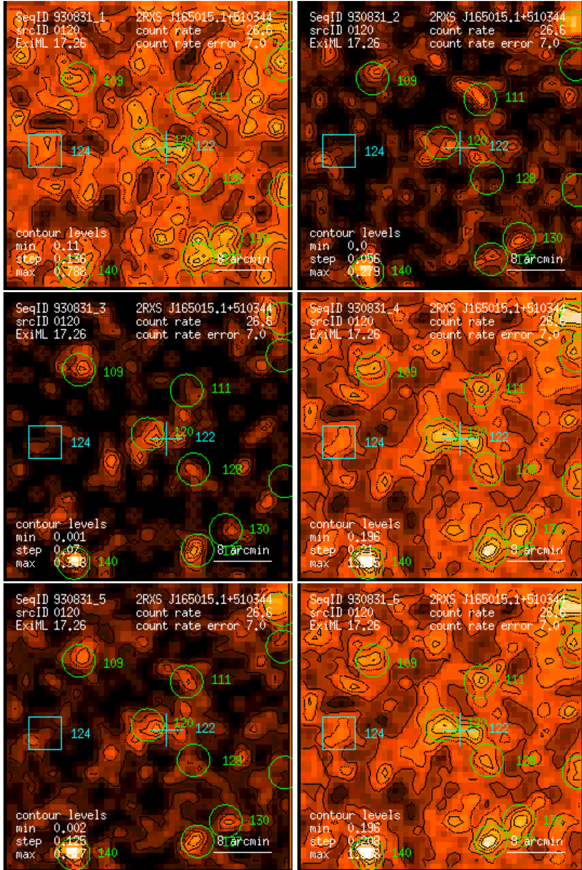
Figure 120: RASS 930831: detection 0120: band rate images, Gaussian filter: (1) PSPC channels 11 – 41, (2) 52 – 90, (3) 91 – 201, (4) 11 – 235, (5) 52 – 201, (6) 11 – 201. Broad band rates in counts/ks. Band rate contour levels in counts/ks/arcmin 2 .
